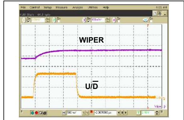
FIGURE 2-26: 5 k \Omega – Low-Voltage Increment Wiper Settling Time ( V_{DD} = 5.5\text{V} ).
