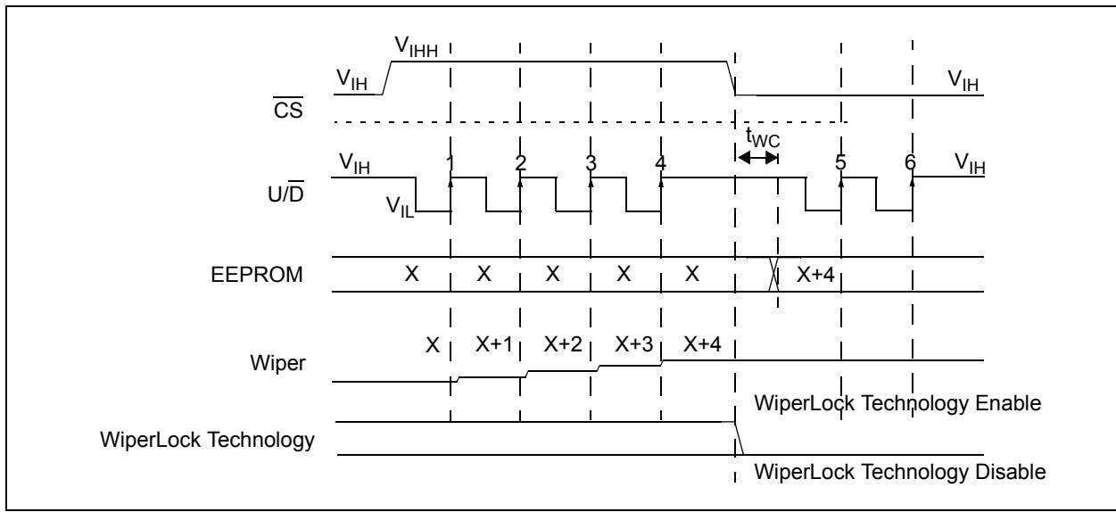
FIGURE 5-6: High-Voltage Increment and Disable WiperLock Technology.
