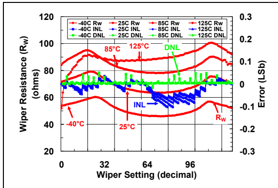
FIGURE 2-57: 100 kΩ Pot Mode : R_W ( \Omega ), INL (LSb), DNL (LSb) vs. Wiper Setting and Temperature ( V_{DD} = 5\text{V} ).
