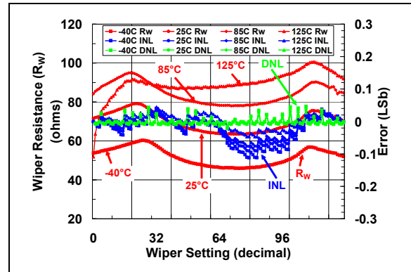
FIGURE 2-60: 100 kΩ Rheo Mode : R_W ( \Omega ), INL (LSb), DNL (LSb) vs. Wiper Setting and Temperature ( V_{DD} = 5\text{V} ). ( I_W = 45\mu\text{A} , B = V_{SS} )
