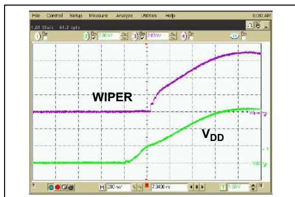
FIGURE 2-15: 2.1 k \Omega – Power-Up Wiper Response Time.
