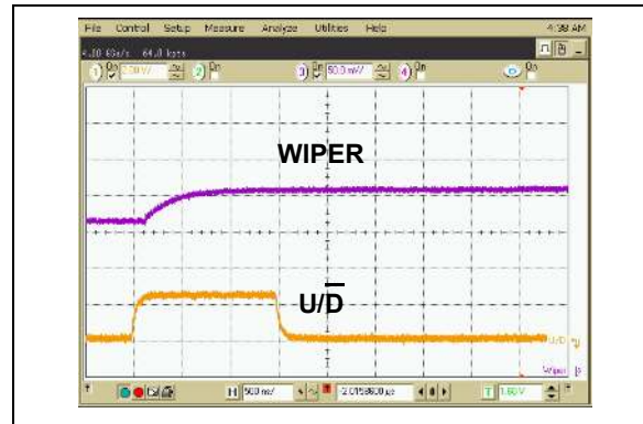
FIGURE 2-28: 5 k \Omega – Low-Voltage Increment Wiper Settling Time ( V_{DD} = 2.7\text{V} ).
