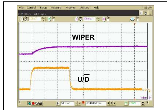
FIGURE 2-29: 5 k \Omega – Low-Voltage Increment Wiper Settling Time ( V_{DD} = 5.5\text{V} ).
