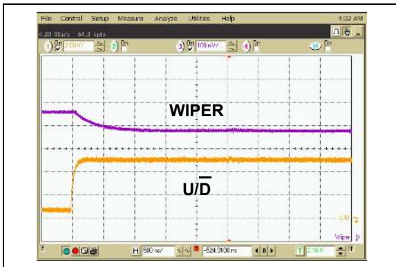
FIGURE 2-27: 5 k \Omega – Low-Voltage Decrement Wiper Settling Time ( V_{DD} = 5.5\text{V} ).
