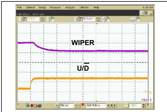
FIGURE 2-26: 5 k \Omega – Low-Voltage Decrement Wiper Settling Time ( V_{DD} = 2.7\text{V} ).
