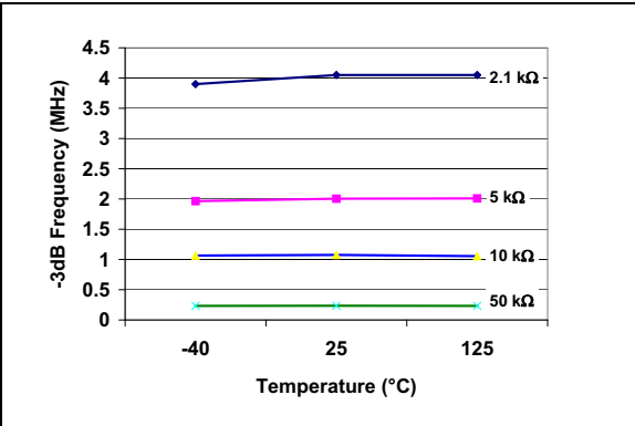
FIGURE 2-55: -3\text{ dB} Bandwidth vs. Temperature.
