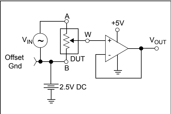
FIGURE 2-56: -3\text{ dB} Bandwidth Test Circuit.
