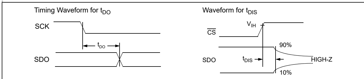
FIGURE 1-4: Timing Waveforms.
