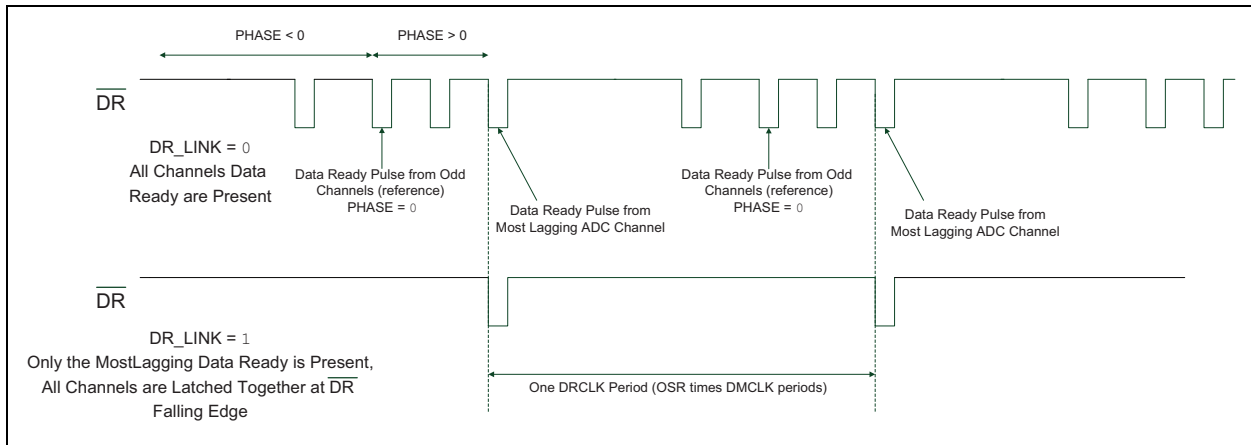
FIGURE 5-8: DR_LINK Configurations.
