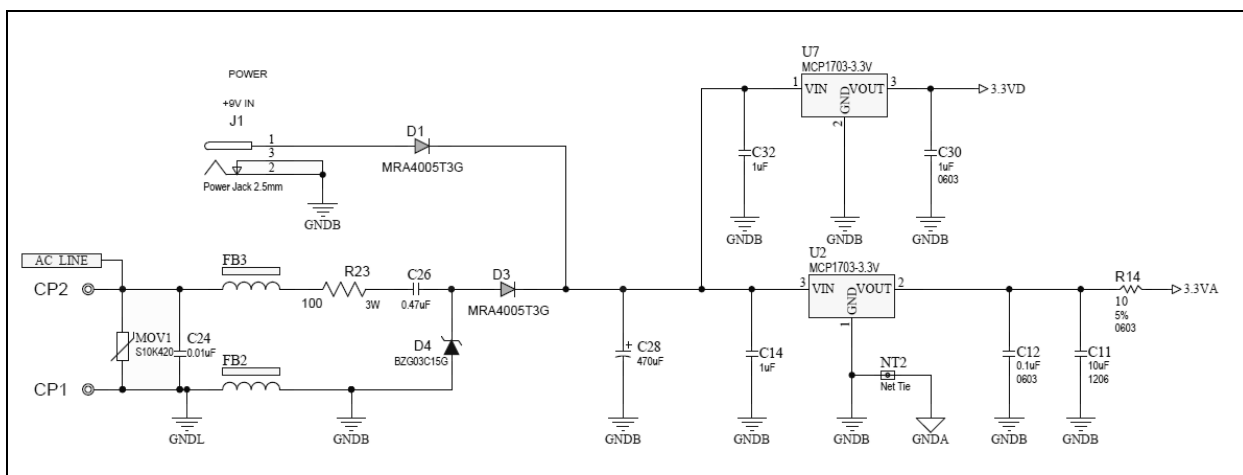
FIGURE 8-3: Power Supply with Separate Lines for Analog and Digital Sections. Note the “Net Tie” Object NT2 that Represents the Start Ground Connection.
