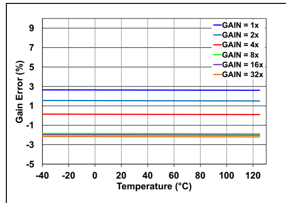
FIGURE 2-35: Gain Error vs. Temperature vs. Gain.
