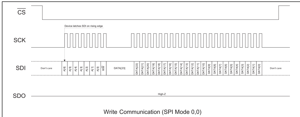
FIGURE 6-5: Write to a Single Register with 24-Bit Format ( WIDTH\_CRC = 0 , SPI Mode 0,0).
