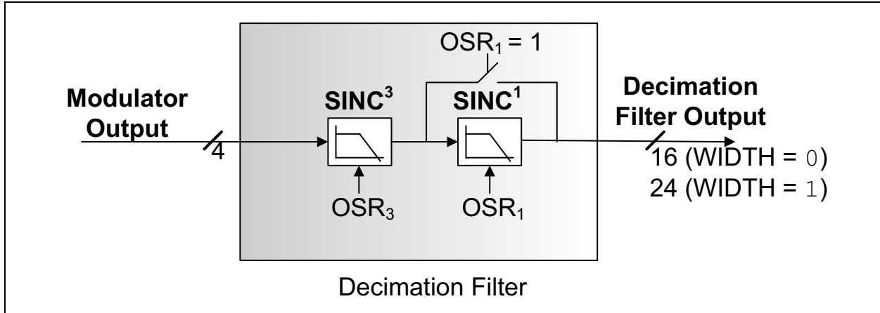
FIGURE 5-3: MCP3918B Decimation Filter Block Diagram.
