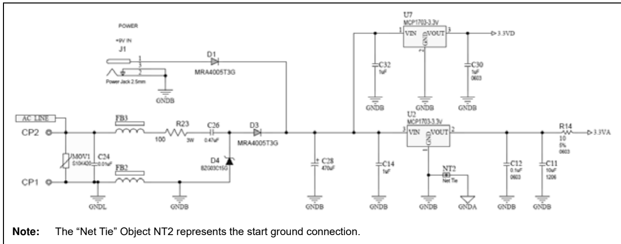
FIGURE 8-3: Power Supply with Separate Lines for Analog and Digital Sections.
