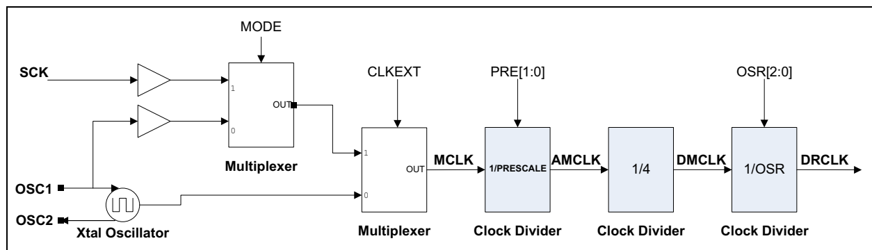
FIGURE 4-1: Clock Subcircuitry.
