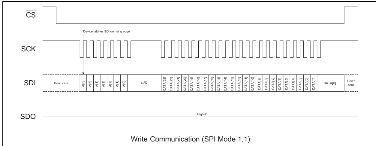
FIGURE 6-4: Write to a Single Register with 24-Bit Format ( WIDTH\_CRC = 0 , SPI Mode 1,1).
