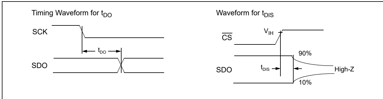
FIGURE 1-4: Timing Waveforms.
