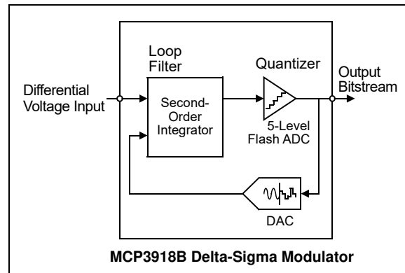
FIGURE 5-1: Simplified Delta-Sigma ADC Block Diagram.
