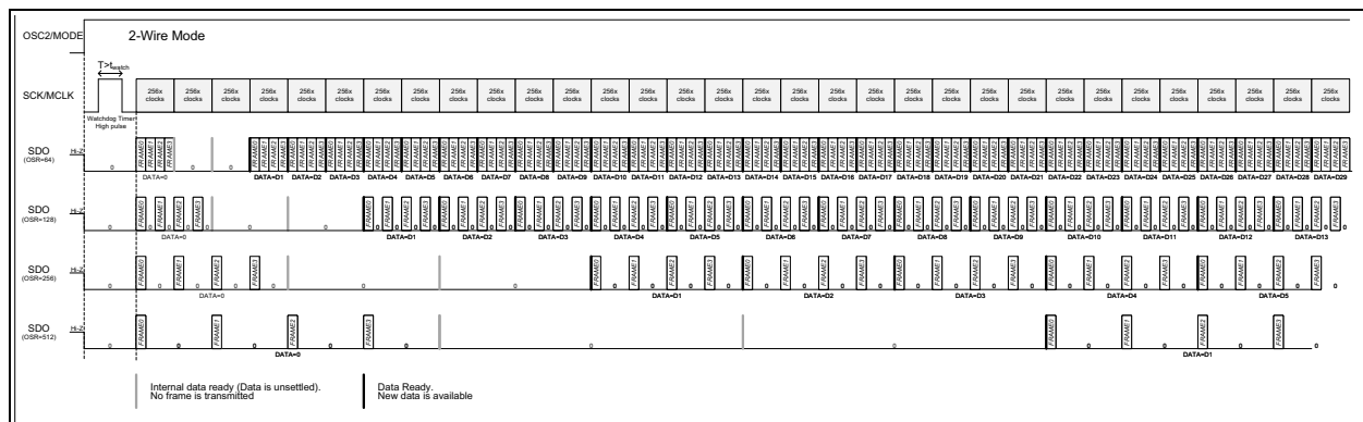
FIGURE 7-3: MCP3918B Two-Wire Communication Protocol.
