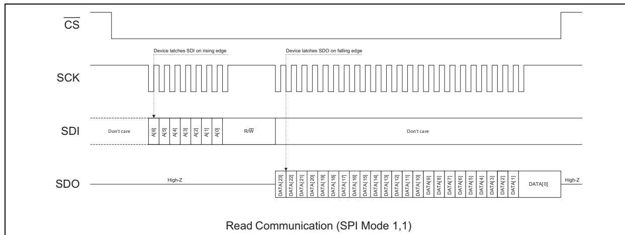
FIGURE 6-2: Read on a Single Register with 24-Bit Format ( WIDTH\_DATA[1:0] = 01 , SPI Mode 1,1).
