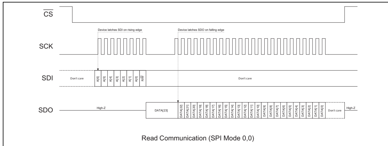
FIGURE 6-3: Read on a Single Register with 24-Bit Format ( WIDTH\_DATA[1:0] = 01 , SPI Mode 0,0).
