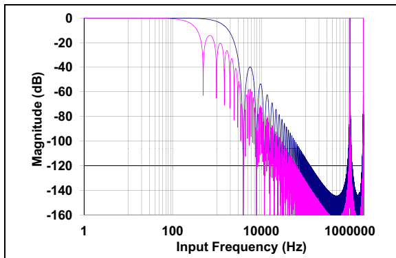
FIGURE 5-5: SINC Filter Frequency Response, OSR = 4096 (in pink), OSR = 512 (in blue), MCLK = 4\text{ MHz} , PRE[1:0] = 00 .
