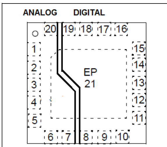
FIGURE 8-4: Separation of Analog and Digital Circuits on Layout.
