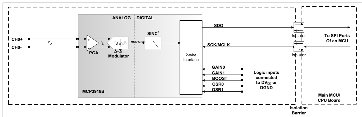
FIGURE 7-1: MCP3918B Two-Wire Interface Typical Application Schematic.
