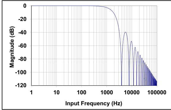
FIGURE 5-4: SINC Filter Frequency Response, OSR = 256 , MCLK = 4\text{ MHz} , PRE[1:0] = 00 .
