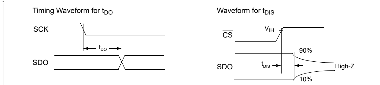
FIGURE 1-4: Timing Waveforms.
