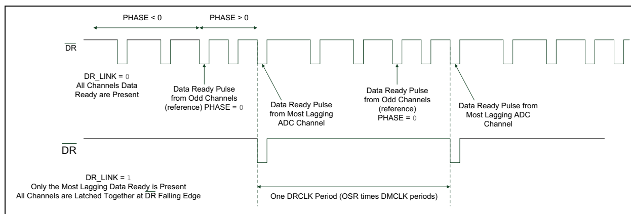
FIGURE 5-8: DR_LINK Configurations.
