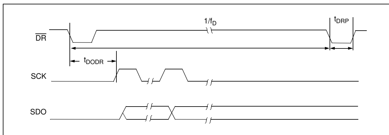
FIGURE 1-3: Data Ready Pulse/Sampling Timing Diagram.
