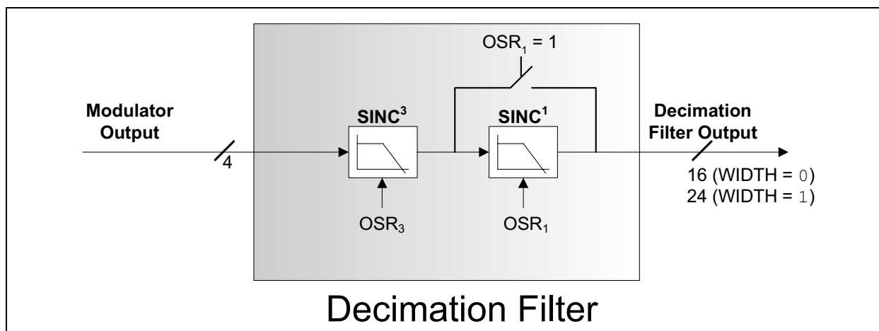
FIGURE 5-3: MCP3911 Decimation Filter Block Diagram.
