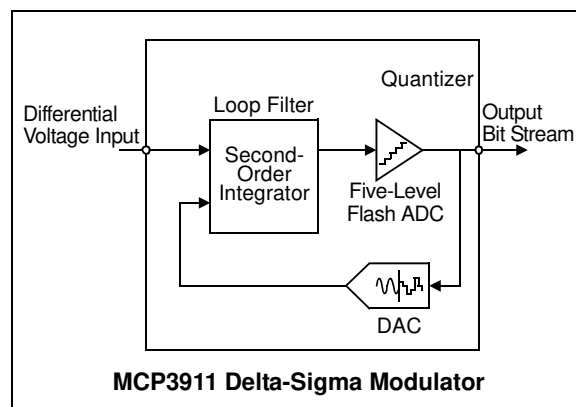
FIGURE 5-1: Simplified Delta-Sigma ADC Block Diagram.
