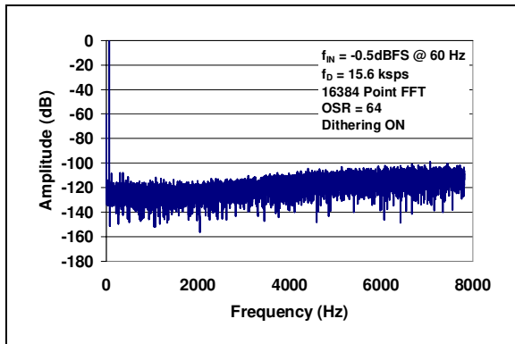
FIGURE 2-7: Spectral Response.
