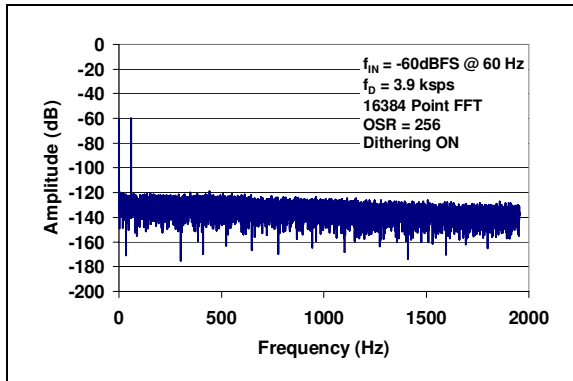
FIGURE 2-2: Spectral Response.
