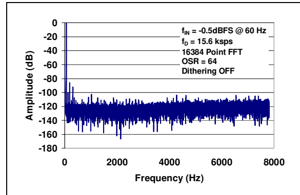
FIGURE 2-5: Spectral Response.
