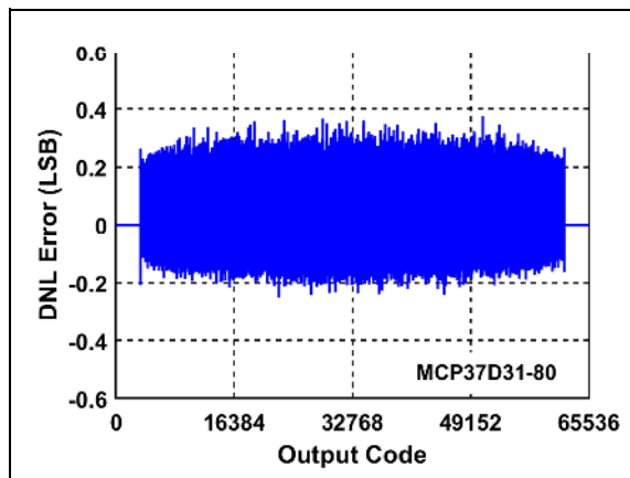
FIGURE 3-43: DNL Error Vs. Output Code: f_S = 80 \text{ Msps} , f_{IN} = 4.3 \text{ MHz} , A_{IN} = -1\text{dBFS} , MCP37D31-80.
