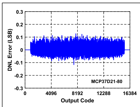
FIGURE 3-44: DNL Error Vs. Output Code: f_S = 80 \text{ Msps} , f_{IN} = 4.3 \text{ MHz} , A_{IN} = -1\text{dBFS} , MCP37D21-80.
