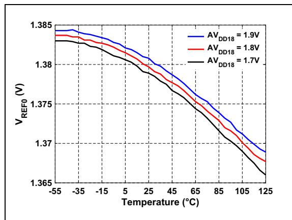
FIGURE 3-38: V_{REF0} vs. Temperature.
