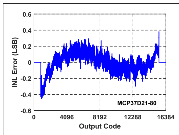
FIGURE 3-41: INL Error Vs. Output Code: f_S = 80 \text{ Msps} , f_{IN} = 4.3 \text{ MHz} , A_{IN} = -1\text{dBFS} , MCP37D21-80.
