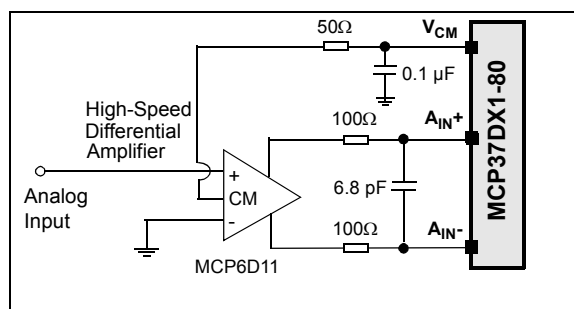
FIGURE 4-4: DC-Coupled Input Configuration with Preamplifier: the external signal conditioning circuit and associated component values are for reference only. Typically, the amplifier manufacturer provides reference circuits and component values.
