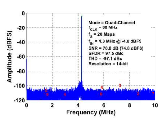
FIGURE 3-18: FFT for 4.3 MHz Input Signal: f_S = 20 Msps, Quad-Ch., A_{IN} = -4 dBFS.
