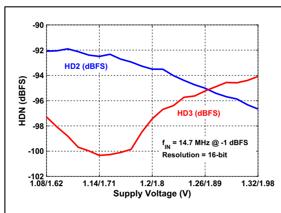
FIGURE 3-39: HD2/HD3 vs. Supply Voltage: f_S = 80 Msps, f_{IN} = 14.7 MHz.
