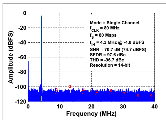
FIGURE 3-16: FFT for 4.3 MHz Input Signal: f_S = 80 Msps, Single-Ch., A_{IN} = -4 dBFS.
