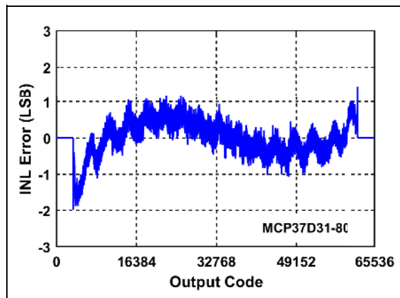
FIGURE 3-40: INL Error Vs. Output Code: f_S = 80 \text{ Msps} , f_{IN} = 4.3 \text{ MHz} , A_{IN} = -1\text{dBFS} , MCP37D31-80.
