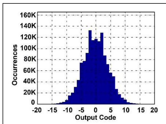
FIGURE 3-42: Shorted Input Histogram: f_S = 80 \text{ Msps} , MCP37D31-80.
