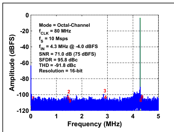
FIGURE 3-10: FFT for 4.3 MHz Input Signal: f_S = 10 Msps, Octal-Ch., A_{IN} = -4 dBFS.
