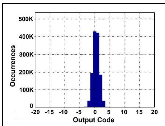
FIGURE 3-45: Shorted Input Histogram: f_S = 80 \text{ Msps} , MCP37D21-80.
