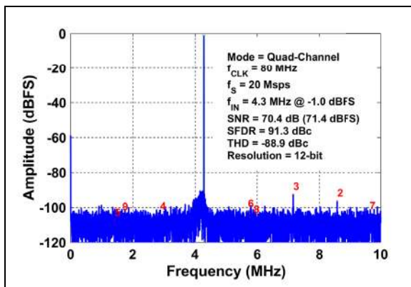
FIGURE 3-3: FFT for 4.3 MHz Input Signal: f_S = 20 Mps, Quad-Ch., A_{IN} = -1 dBFS.
