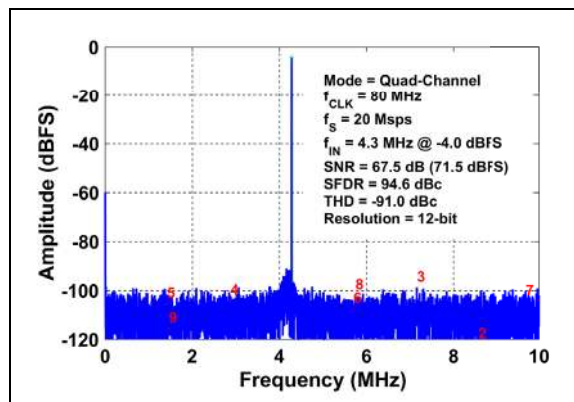
FIGURE 3-6: FFT for 4.3 MHz Input Signal: f_S = 20 Mps, Quad-Ch., A_{IN} = -4 dBFS.
