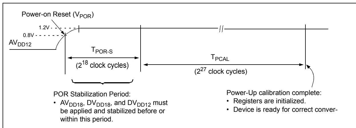
FIGURE 2-5: Internal Power-Up Sequence Events.
