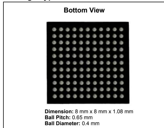
TFBGA-121 Package
