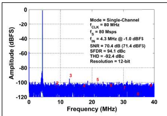
FIGURE 3-1: FFT for 4.3 MHz Input Signal: f_S = 80 Mps, Single-Ch., A_{IN} = -1 dBFS.
