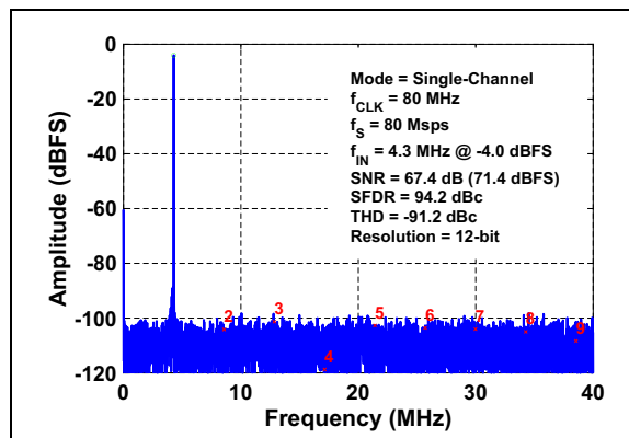
FIGURE 3-4: FFT for 4.3 MHz Input Signal: f_S = 80 Mps, Single Ch., A_{IN} = -4 dBFS.
