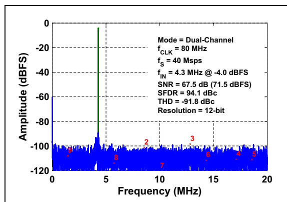
FIGURE 3-5: FFT for 4.3 MHz Input Signal: f_S = 40 Mps, Dual-Ch., A_{IN} = -4 dBFS.
