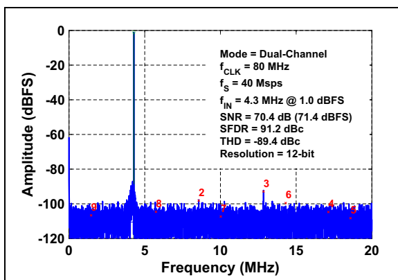
FIGURE 3-2: FFT for 4.3 MHz Input Signal: f_S = 40 Mps, Dual-Ch., A_{IN} = -1 dBFS.
