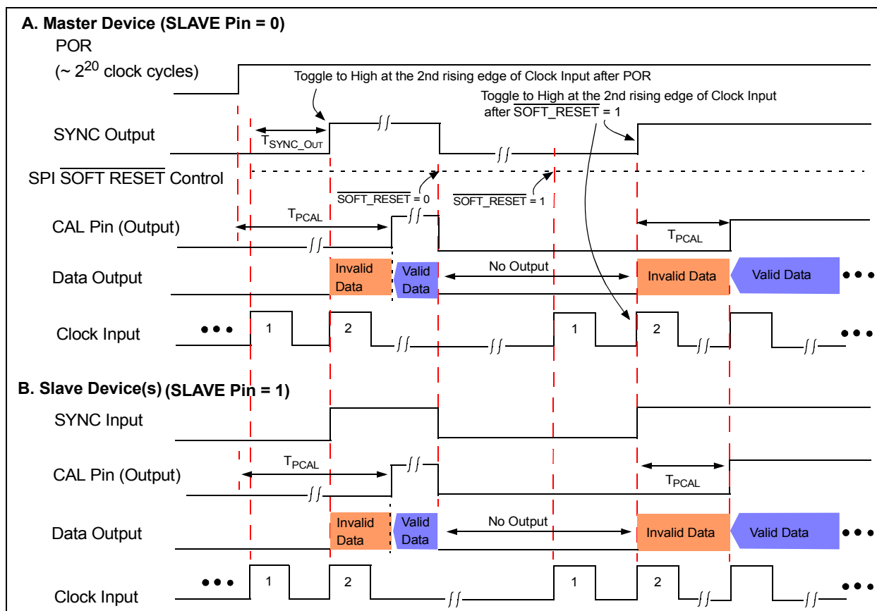
FIGURE 2-11: Sync Timing Diagram with SOFT\_RESET Bit Setting.
