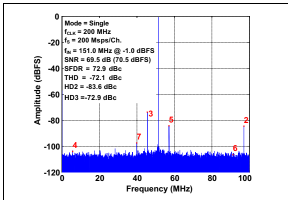
FIGURE 3-3: FFT for 151 MHz Input Signal: f_S = 200 Mps/Ch., A_{IN} = -1 dBFS.
