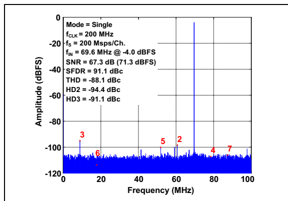
FIGURE 3-5: FFT for 69.6 MHz Input Signal: f_S = 200 Mps/Ch., A_{IN} = -4 dBFS.
