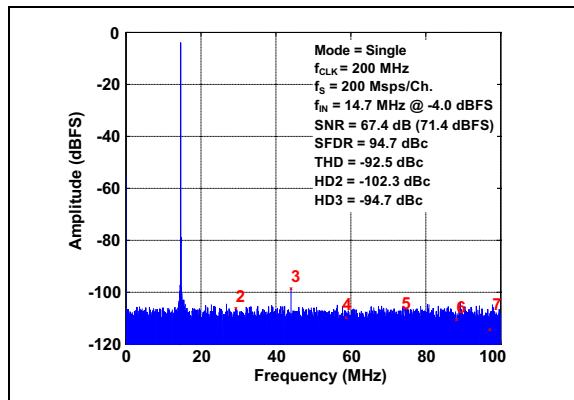
FIGURE 3-4: FFT for 14.7 MHz Input Signal: f_S = 200 Mps/Ch., A_{IN} = -4 dBFS.
