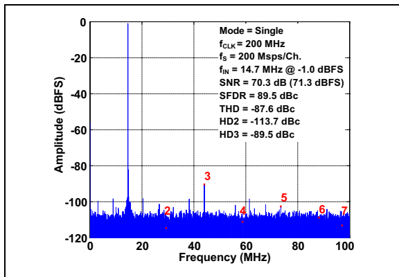
FIGURE 3-1: FFT for 14.7 MHz Input Signal: f_S = 200 Mps/Ch., A_{IN} = -1 dBFS.
