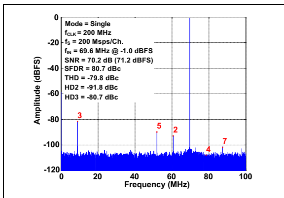
FIGURE 3-2: FFT for 69.6 MHz Input Signal: f_S = 200 Mps/Ch., A_{IN} = -1 dBFS.
