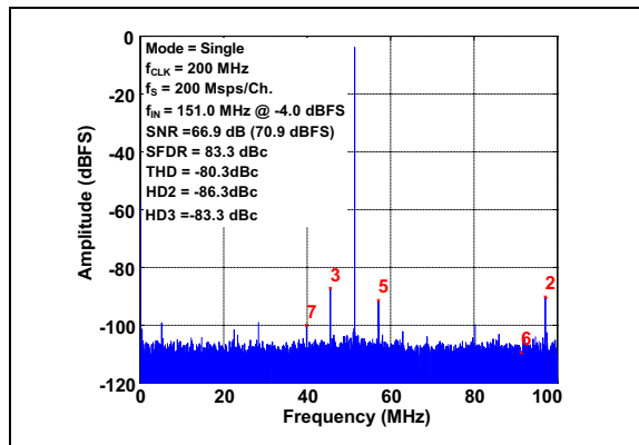
FIGURE 3-6: FFT for 151 MHz Input Signal: f_S = 200 Mps/Ch., A_{IN} = -4 dBFS.
