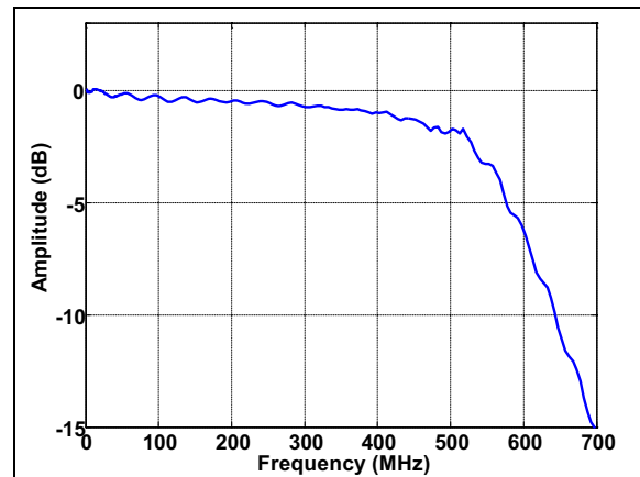
FIGURE 3-44: Input Bandwidth.
