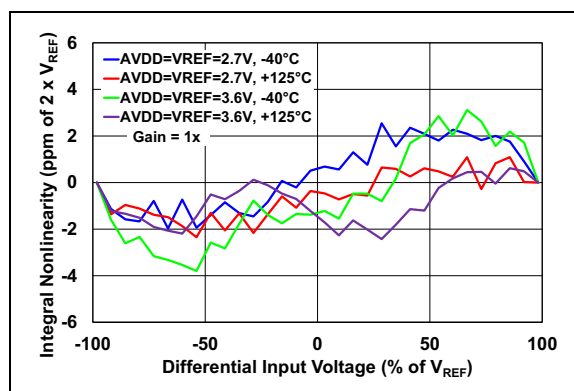
FIGURE 2-4: INL vs. Input Voltage.
