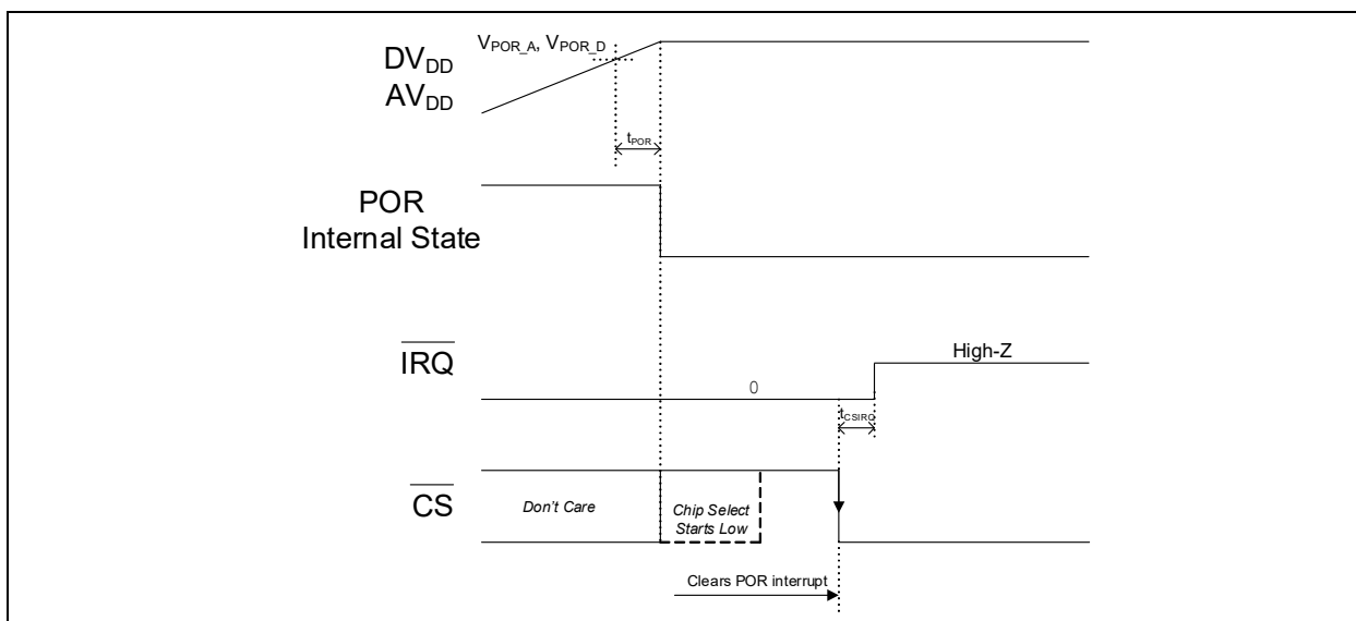
FIGURE 6-15: POR \overline{\text{IRQ}} Timing Diagram.
