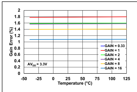
FIGURE 2-31: Gain Error vs. Temperature.
