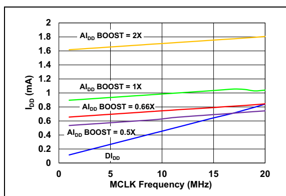
FIGURE 2-36: DI_{DD} and AI_{DD} vs. MCLK.
