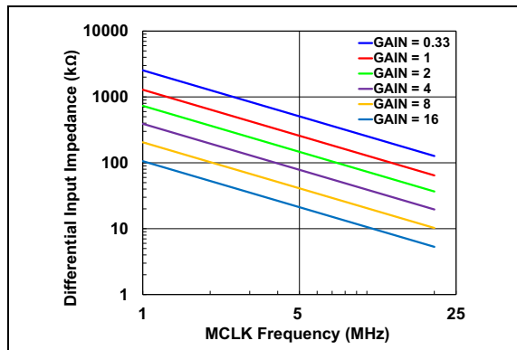
FIGURE 2-34: Differential Input Impedance vs. MCLK.
