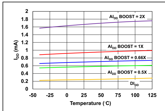
FIGURE 2-38: DI_{DD} and AI_{DD} vs. Temperature.
