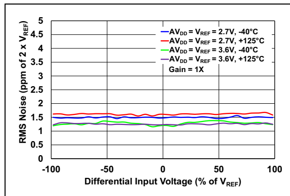
FIGURE 2-5: Output Noise vs. Input Voltage.
