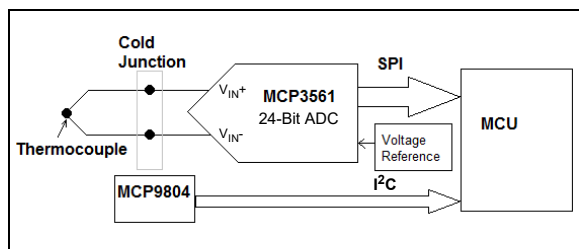
FIGURE 7-2: Thermocouple Connection to MCP3561.
