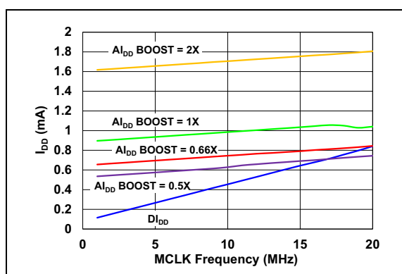
FIGURE 2-36: DI_{DD} and AI_{DD} vs. MCLK.
