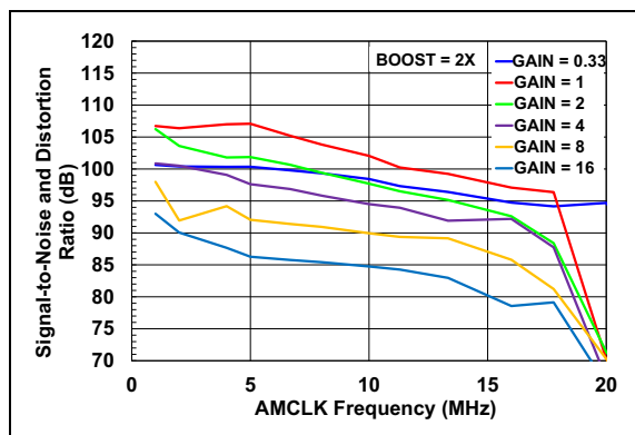
FIGURE 2-23: SINAD vs. AMCLK (BOOST = 2x).
