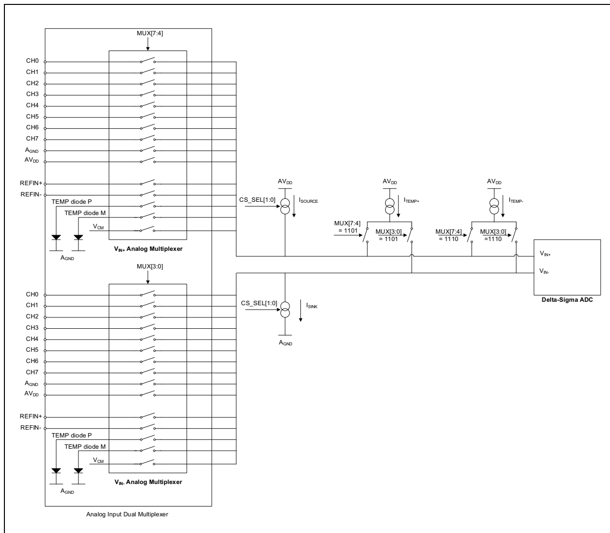
FIGURE 5-1: Simplified Analog Input Multiplexer Schematic.
