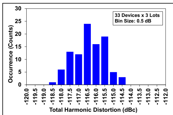
FIGURE 2-20: THD Distribution Histogram External V_{REF} .
