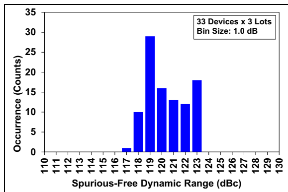
FIGURE 2-21: SFDR Distribution Histogram External V_{REF} .
