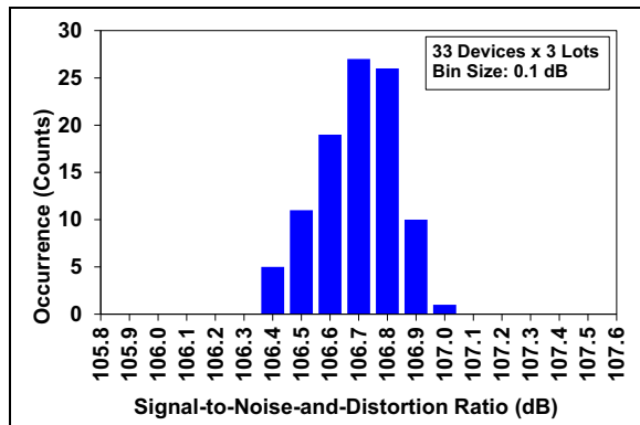
FIGURE 2-19: SINAD Distribution Histogram External V_{REF} .
