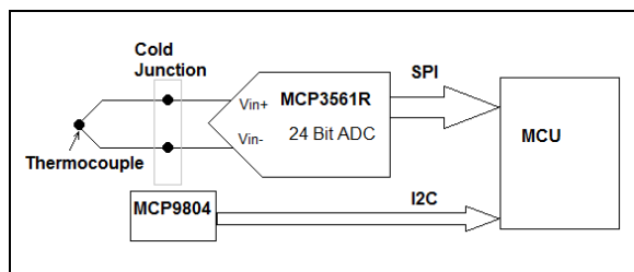
FIGURE 7-2: Thermocouple Connection to MCP3561R.
