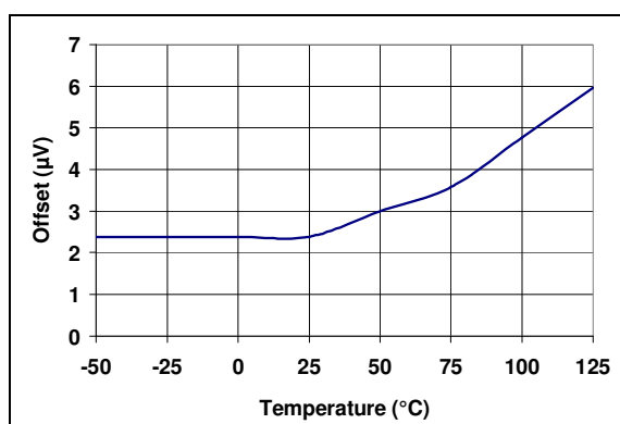
FIGURE 2-12: Offset Error vs. Temperature ( V_{REF} = 5.0\text{V} ).
