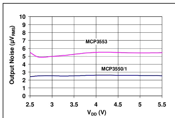
FIGURE 2-9: Output Noise vs. V_{DD} .
