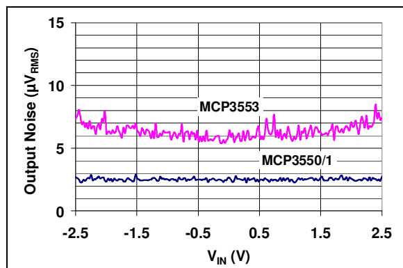
FIGURE 2-7: Output Noise vs. Input Voltage ( V_{DD} = 5.0\text{V} ).
