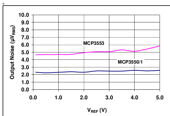
FIGURE 2-8: Output Noise vs. V_{REF} .
