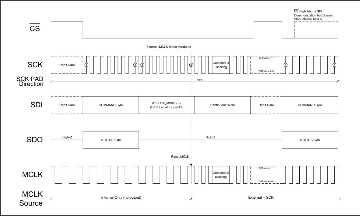
FIGURE 6-13: MCP3465R Transition from CLK_SEL[1:0] = 10 to 0x.
