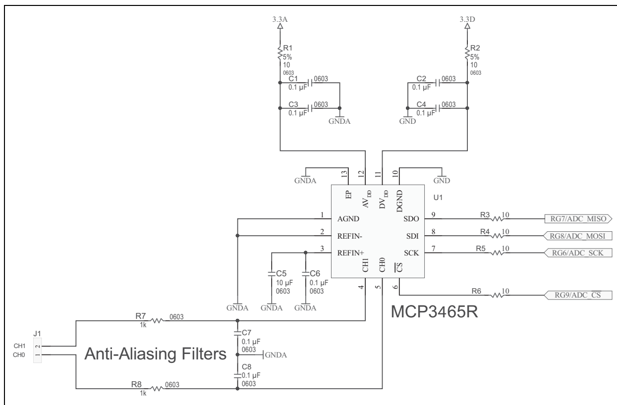
FIGURE 7-1: MCP3465R Application Example.
