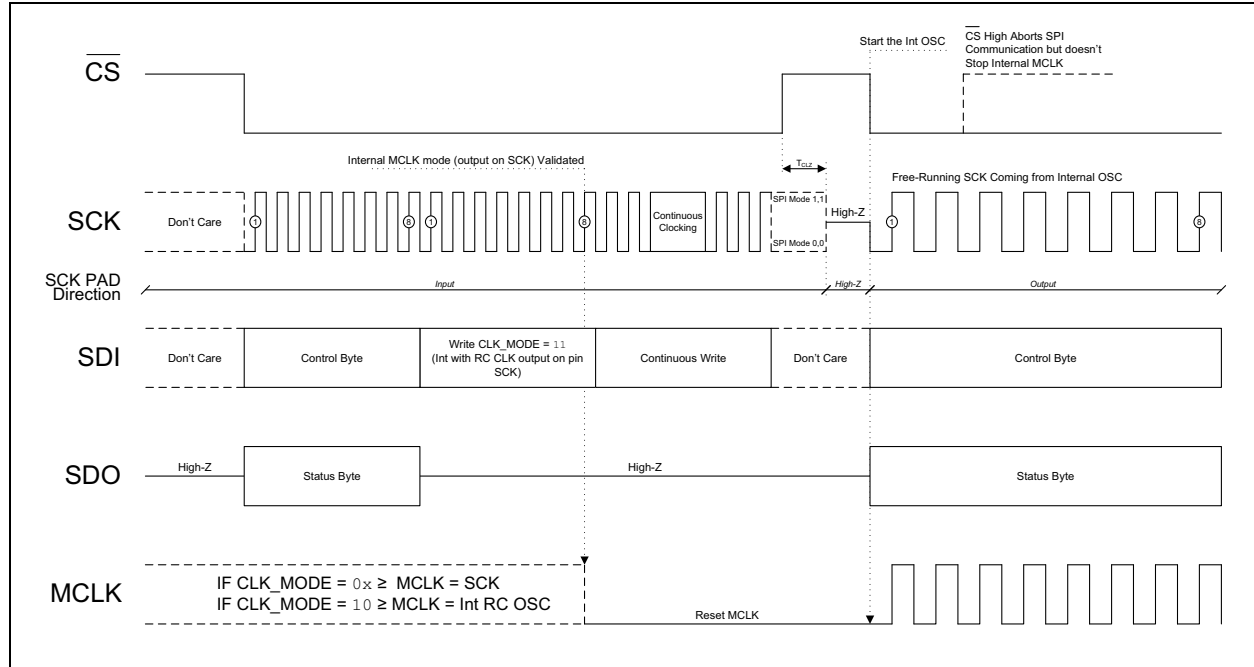
FIGURE 6-15: MCP3465R Transition from CLK_SEL[1:0] = 0x/10 to '11'.
