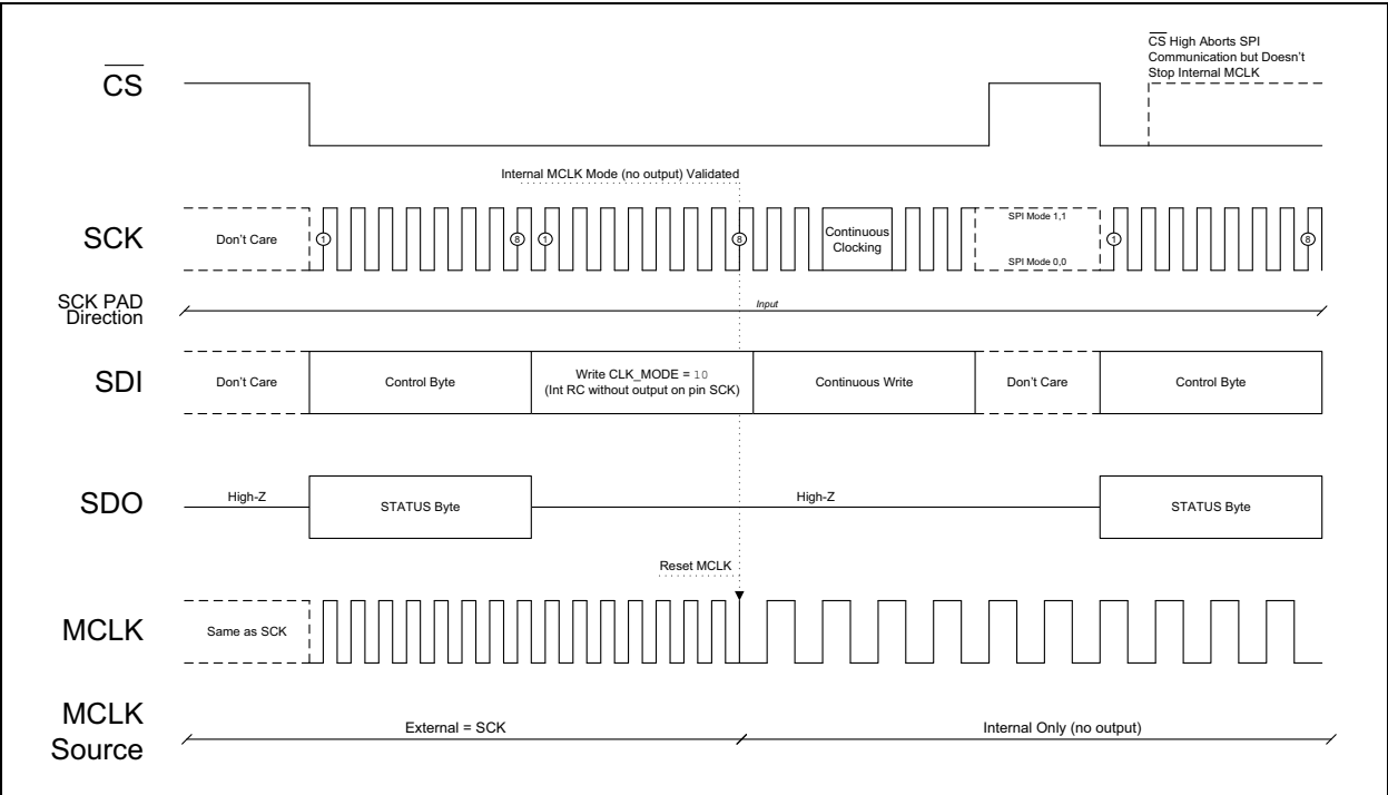
FIGURE 6-14: MCP3465R Transition from CLK_SEL[1:0] = 0x to 10.
