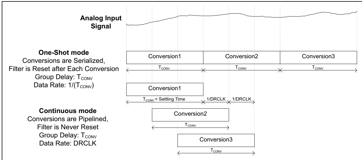
FIGURE 5-5: One-Shot Mode vs. Continuous Mode.
