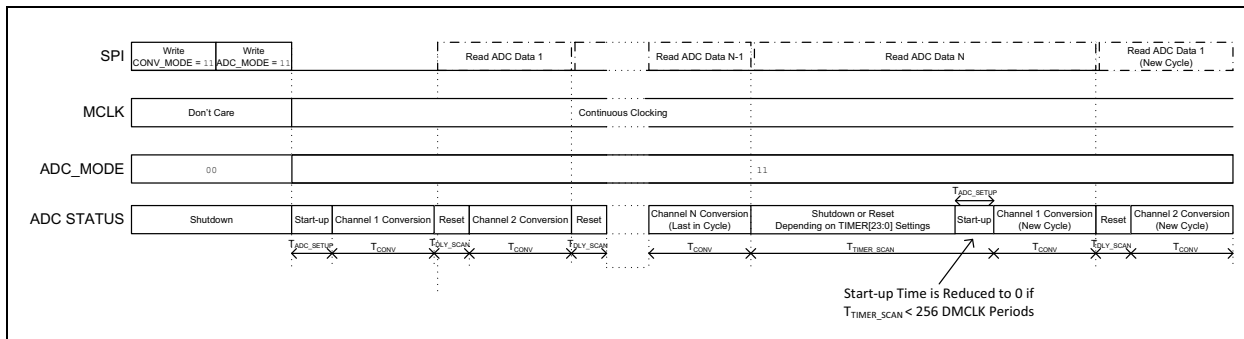
FIGURE 5-17: Scan Continuous Conversion Mode Timing Diagram.
