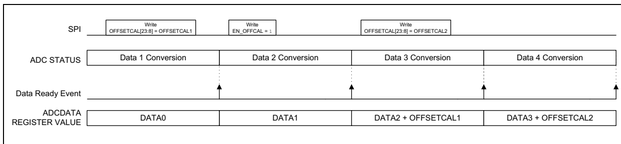
FIGURE 5-12: ADC Output and Data Ready Event Behavior with Digital Offset Calibration Enabled.
