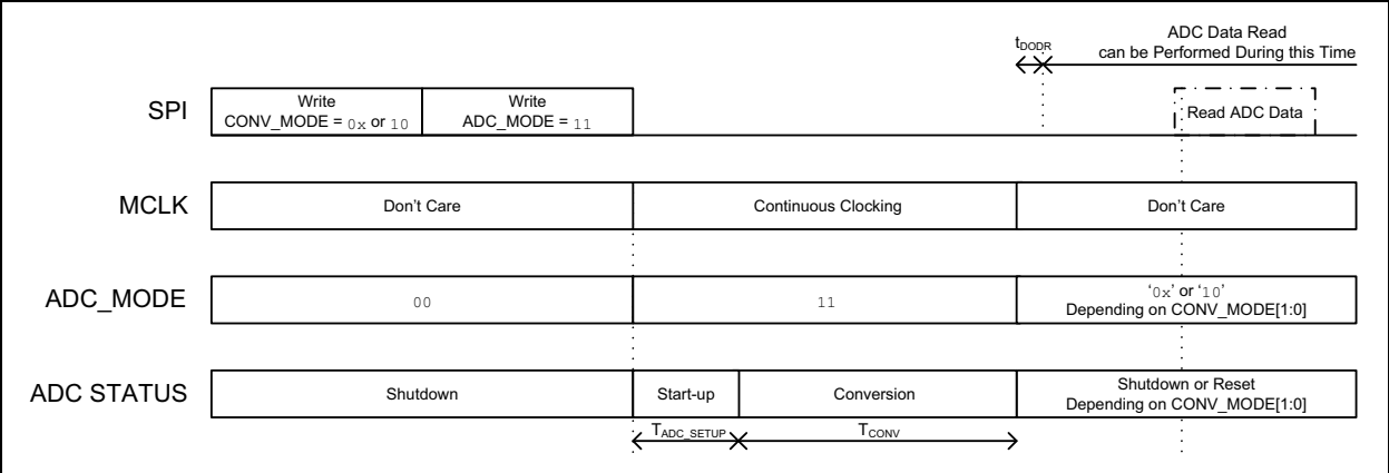
FIGURE 5-14: MUX One-Shot Conversion Mode Timing Diagram.
