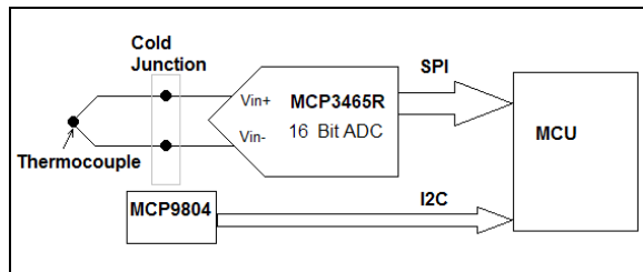
FIGURE 7-2: Thermocouple Connection.
