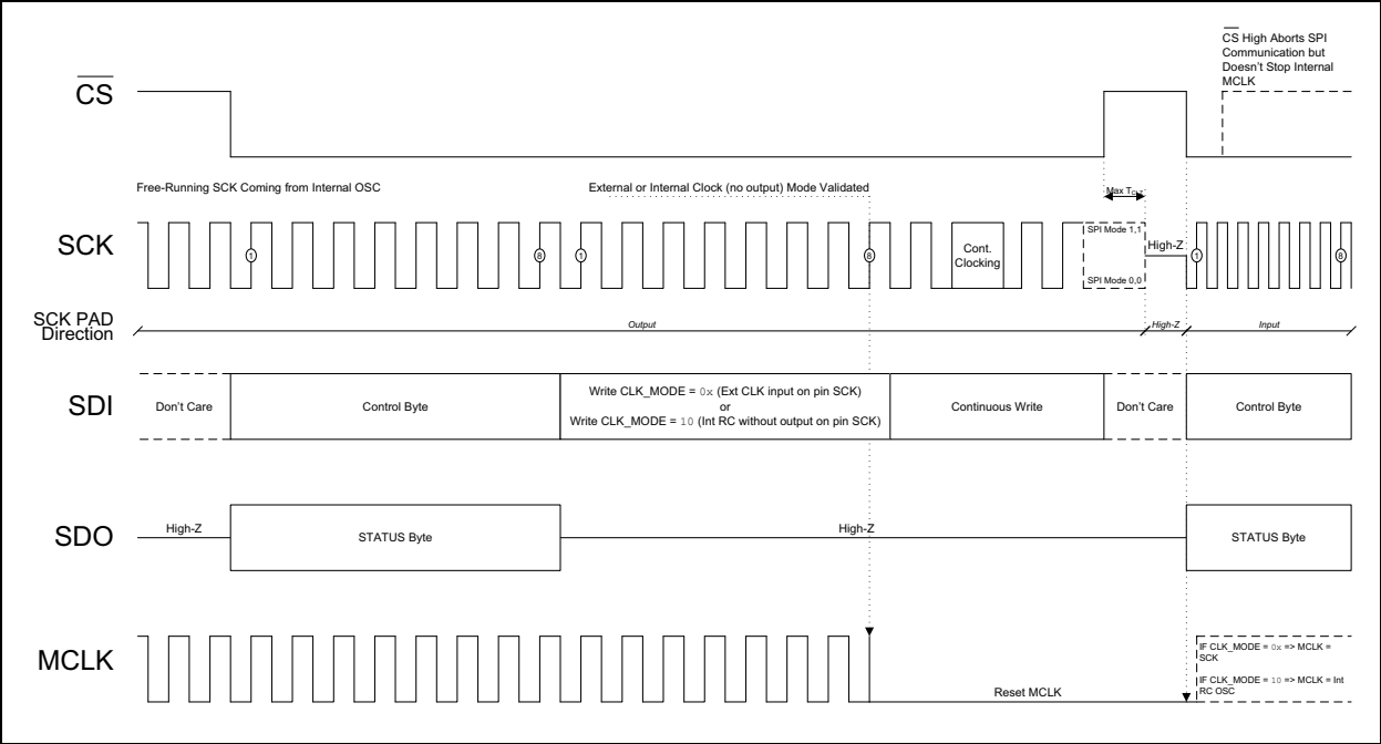
FIGURE 6-16: MCP3465R Transition from CLK_SEL[1:0] = 11 to 0x/10.
