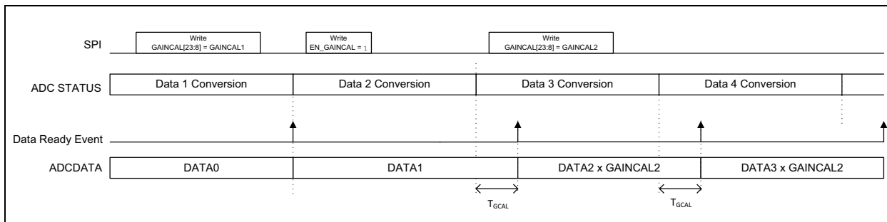
FIGURE 5-13: ADC Output and Data Ready Event Behavior with Digital Gain Error Calibration Enabled.
