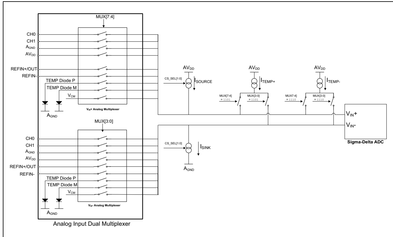
FIGURE 5-1: Simplified Analog Input Multiplexer Schematic.
