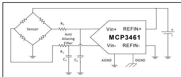
FIGURE 7-3: Wheatstone Bridge Ratiometric Connection.
