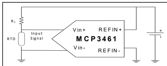
FIGURE 7-4: RTD Ratiometric Connection.
