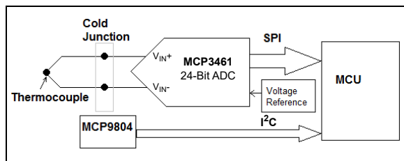
FIGURE 7-2: Thermocouple Connection to MCP3461.
