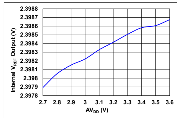
FIGURE 2-60: Internal V_{REF} Output Voltage vs. AV_{DD} .
