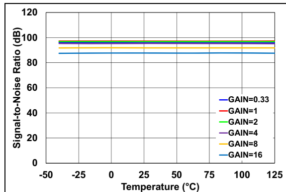
FIGURE 2-16: SNR vs. Temperature.
