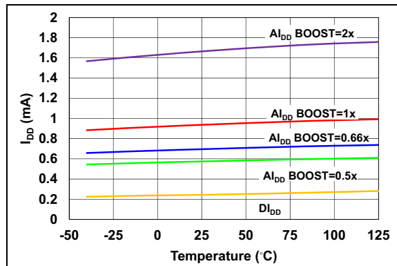
FIGURE 2-38: Current Consumption vs. Temperature.
