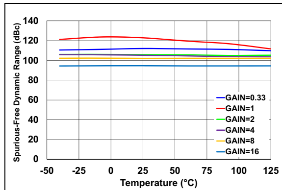
FIGURE 2-18: SFDR vs. Temperature.
