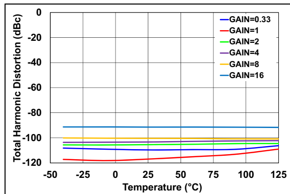
FIGURE 2-17: THD vs. Temperature.
