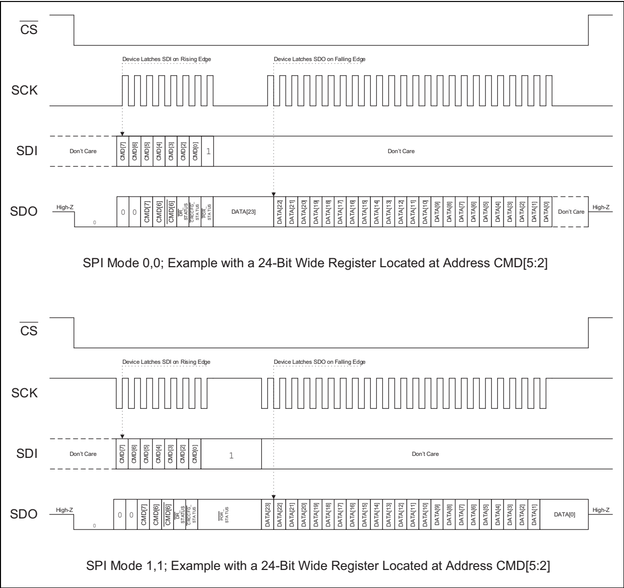
FIGURE 6-8: Single Register Read SPI Communication.
