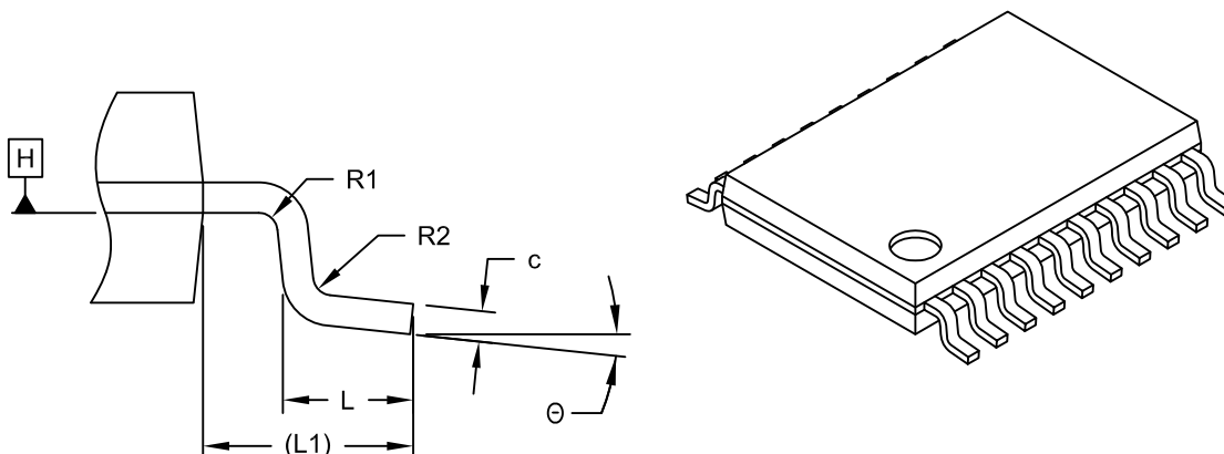
DETAIL B
