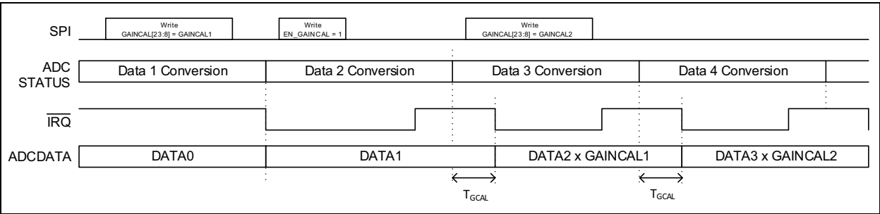
FIGURE 5-12: ADC Output and \overline{IRQ} Behavior with Digital Gain Error Calibration Enabled.
