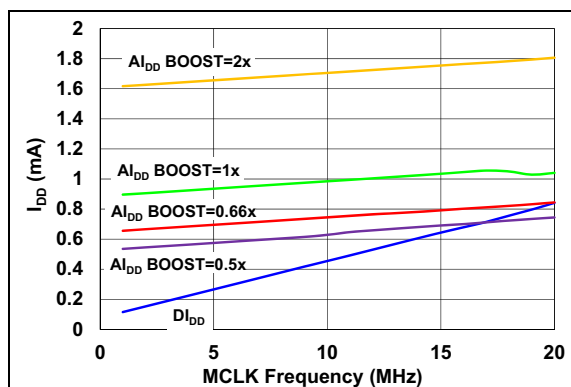
FIGURE 2-36: Current Consumption vs. MCLK.
