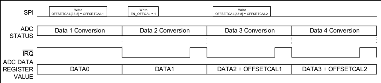
FIGURE 5-11: ADC Output and \overline{IRQ} Behavior with Digital Offset Calibration Enabled.
