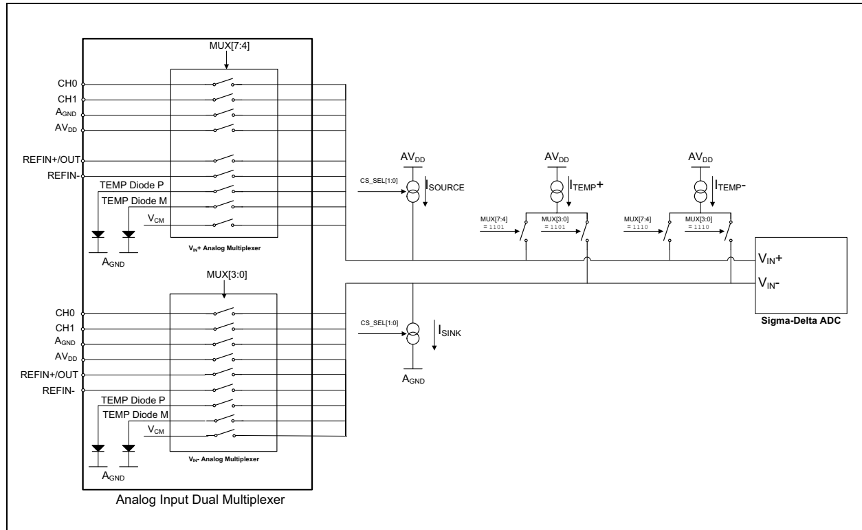
FIGURE 5-1: Simplified Analog Input Multiplexer Schematic.
