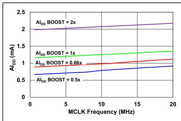
FIGURE 2-56: AI_{DD} vs. MCLK (Internal V_{REF} ).
