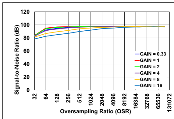
FIGURE 2-11: SNR vs. OSR.
