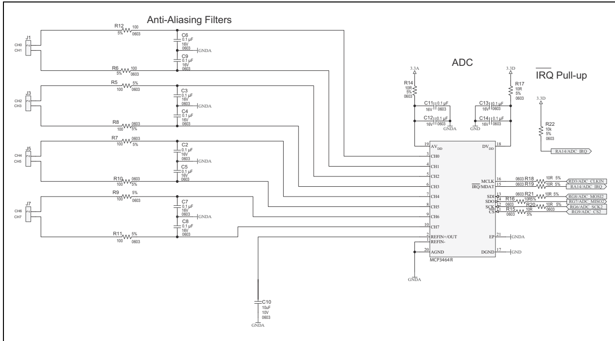
FIGURE 7-1: MCP3464R Application Example.
