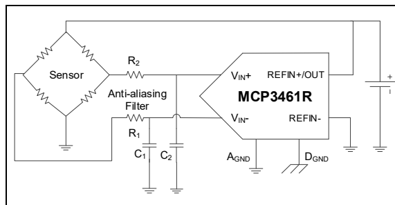
FIGURE 7-4: RTD Ratiometric Connection.
