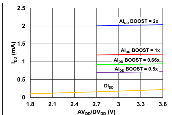
FIGURE 2-55: DI_{DD} and AI_{DD} vs. DV_{DD} and AV_{DD} .
