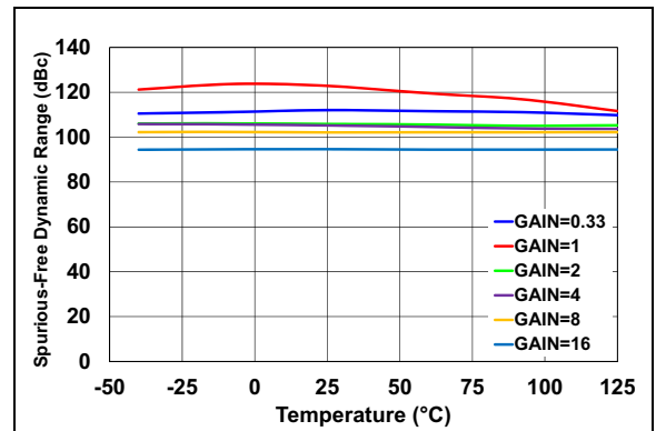
FIGURE 2-29: SFDR vs. Temperature.
