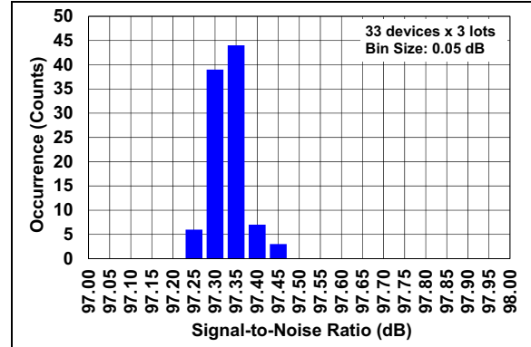
FIGURE 2-18: SNR Distribution Histogram.
