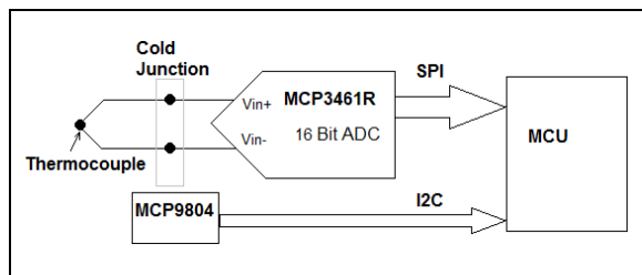
FIGURE 7-2: Thermocouple Connection to MCP3461R.
