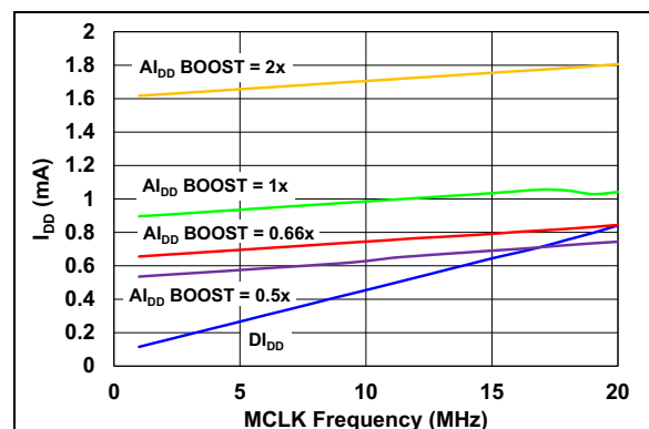
FIGURE 2-54: DI_{DD} and AI_{DD} vs. MCLK.
