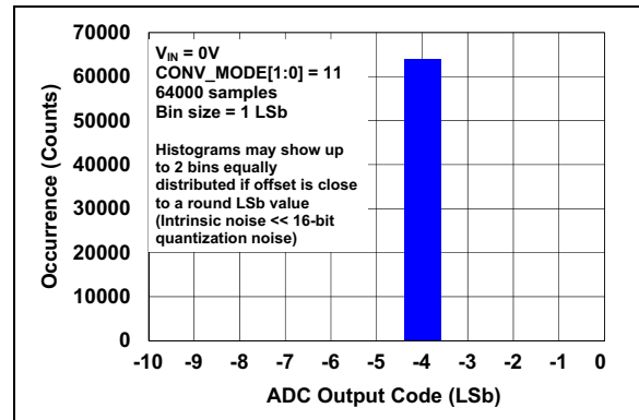
FIGURE 2-5: Output Noise Histogram.
