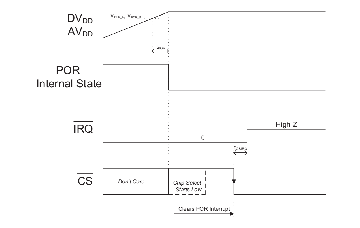
FIGURE 6-16: \text{POR } \overline{\text{IRQ}} Timing Diagram.
