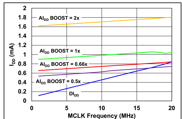
FIGURE 2-54: DI_{DD} and AI_{DD} vs. MCLK .
