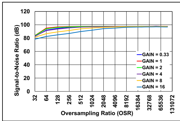
FIGURE 2-11: SNR vs. OSR.
