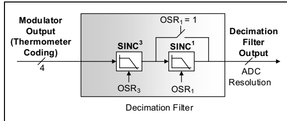
FIGURE 5-4: Decimation Filter Block Diagram.
