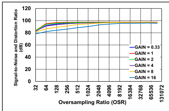
FIGURE 2-10: SINAD vs. OSR.
