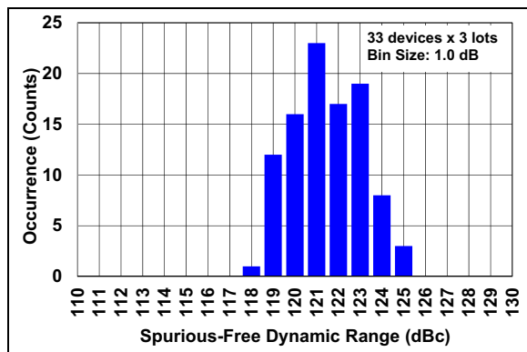
FIGURE 2-21: SFDR Distribution Histogram.
