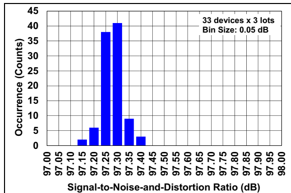
FIGURE 2-19: SINAD Distribution Histogram.
