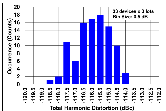
FIGURE 2-20: THD Distribution Histogram.
