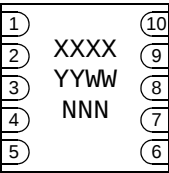
10-Lead DFN (3x3) (MCP3427)
