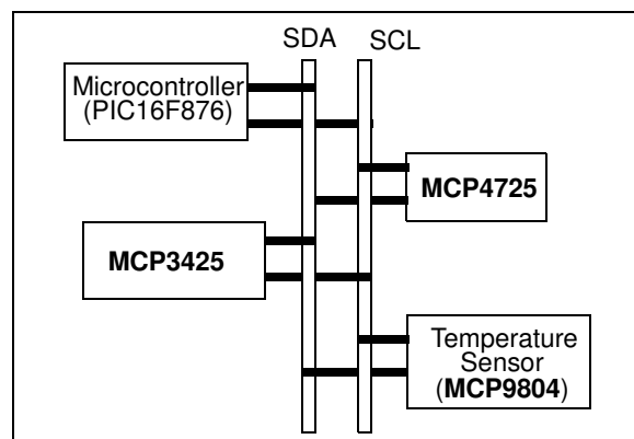
FIGURE 6-2: Example of Multiple Device Connection on I^2C Bus.
