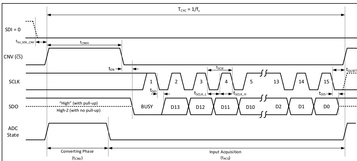
FIGURE 6-7: Timing Diagram for 3-Wire \overline{\text{CS}} Mode with \text{BUSY} Status Indicator Output Bit, Late \text{CNV} .
