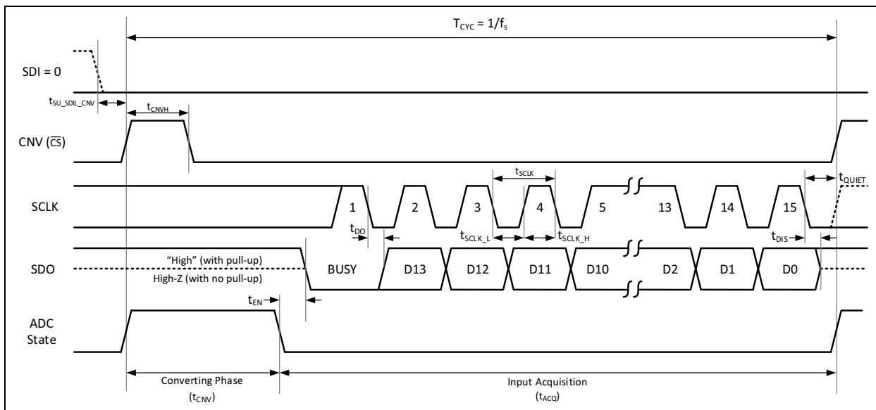
FIGURE 6-6: Timing Diagram for 3-Wire \overline{CS} Mode with BUSY Status Indicator Output Bit, Early CNV (Recommended).
