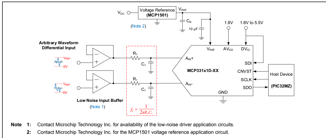
FIGURE 5-4: Input Configuration for Arbitrary Waveform Input Signals.
