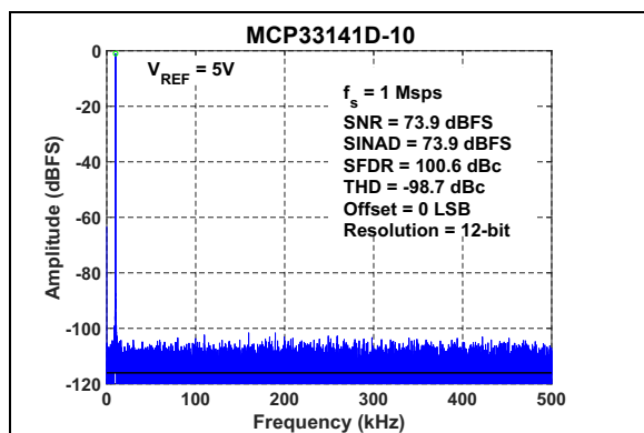
FIGURE 3-8: FFT for 10 kHz Input Signal: f_s = 1\text{ Msp} , V_{IN} = -1\text{ dBFS} , V_{REF} = 5\text{V} .
