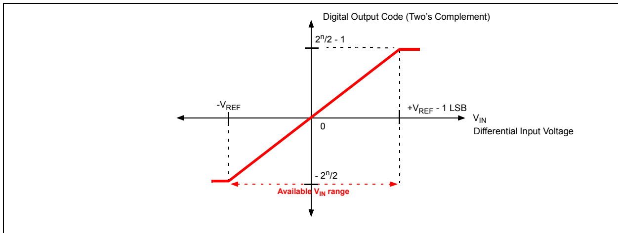
FIGURE 5-3: Transfer Function for Figure 5-2 .
