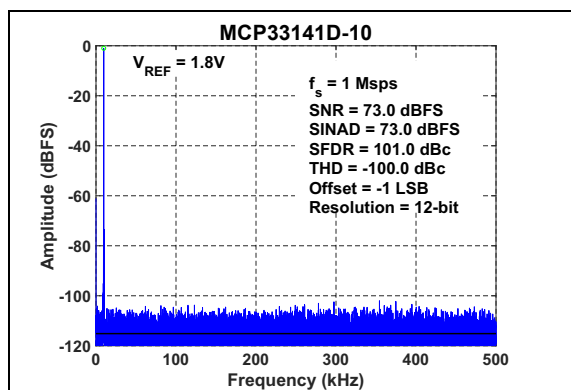
FIGURE 3-11: FFT for 10 kHz Input Signal: f_s = 1\text{ Msp} , V_{IN} = -1\text{ dBFS} , V_{REF} = 1.8\text{V} .
