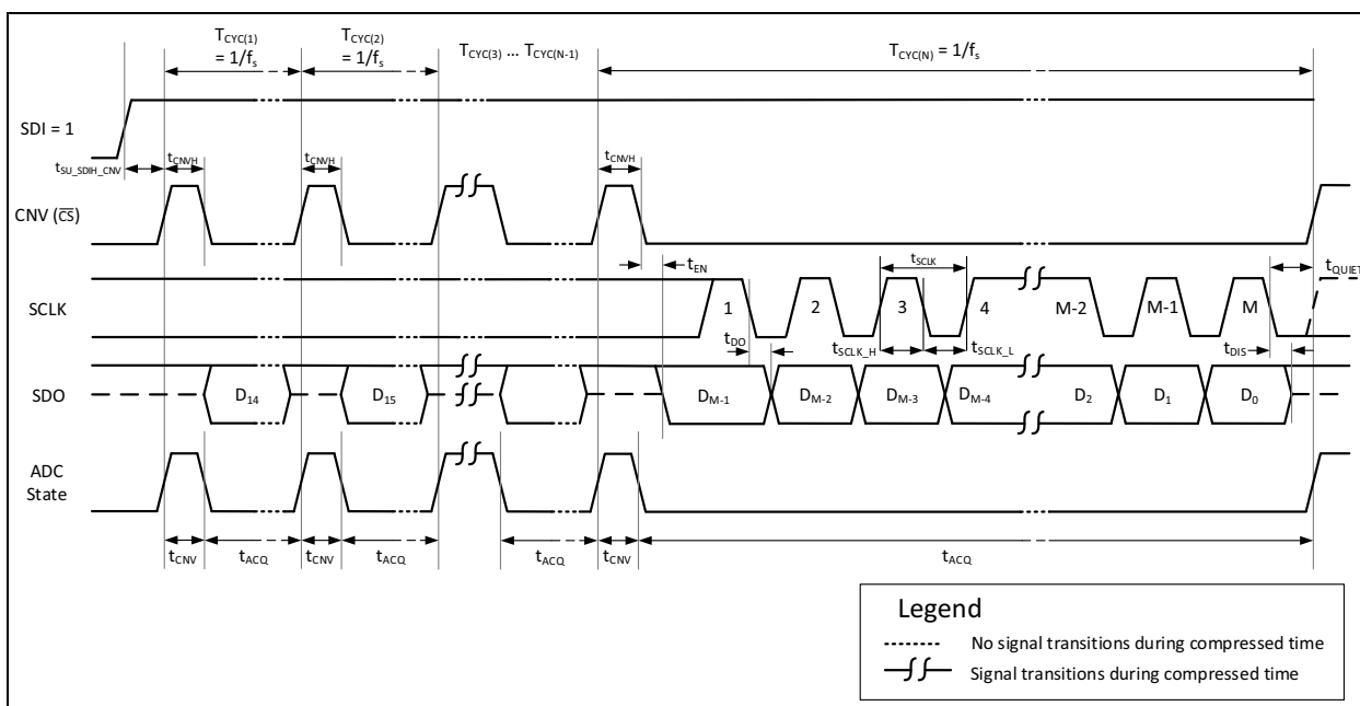
FIGURE 6-4: Interface Timing Diagram for Accumulator Operation in 3-Wire \overline{\text{CS}} Mode without BUSY Status Indicator Output Bit.
