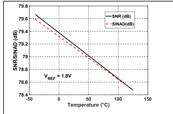
FIGURE 2-17: SNR/SINAD vs. Temperature: V_{REF} = 1.8\text{V} .
