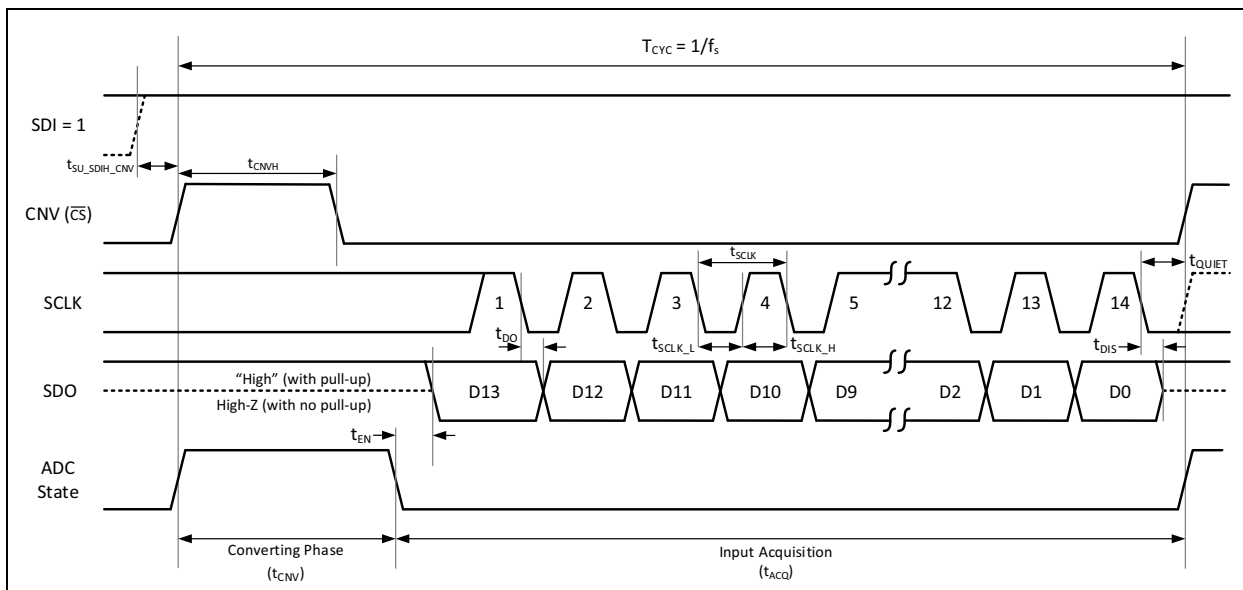
FIGURE 6-3: Interface Timing Diagram for 3-Wire \overline{\text{CS}} Mode without BUSY Status Indicator Output Bit, Early CNV.
