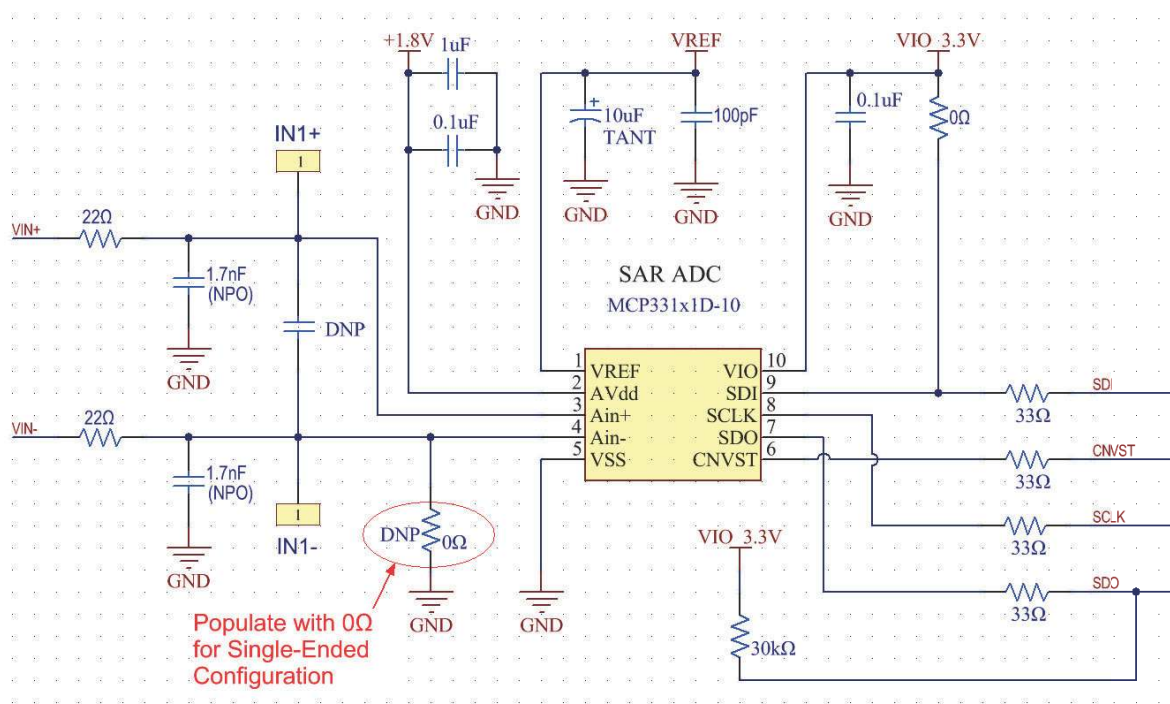
(b) Schematic example from the MCP331x1D-XX Evaluation Board
