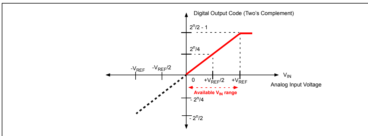
FIGURE 5-7: Pseudo-Differential Unipolar-Input Configuration for Single-Ended Input Signal.
