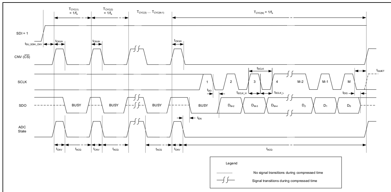
FIGURE 6-8: Interface Timing Diagram for Accumulator Operation in 3-Wire \text{CS} Mode, with \text{BUSY} Status Indicator Output Bit.
