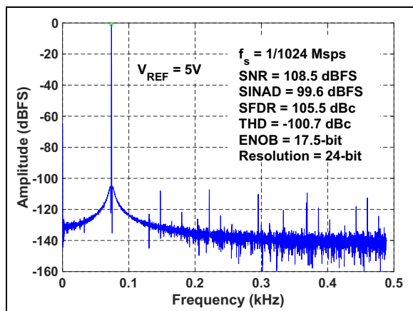
FIGURE 5-7: FFT with 1024 Integrated Samples: Input Freq = 75Hz.
