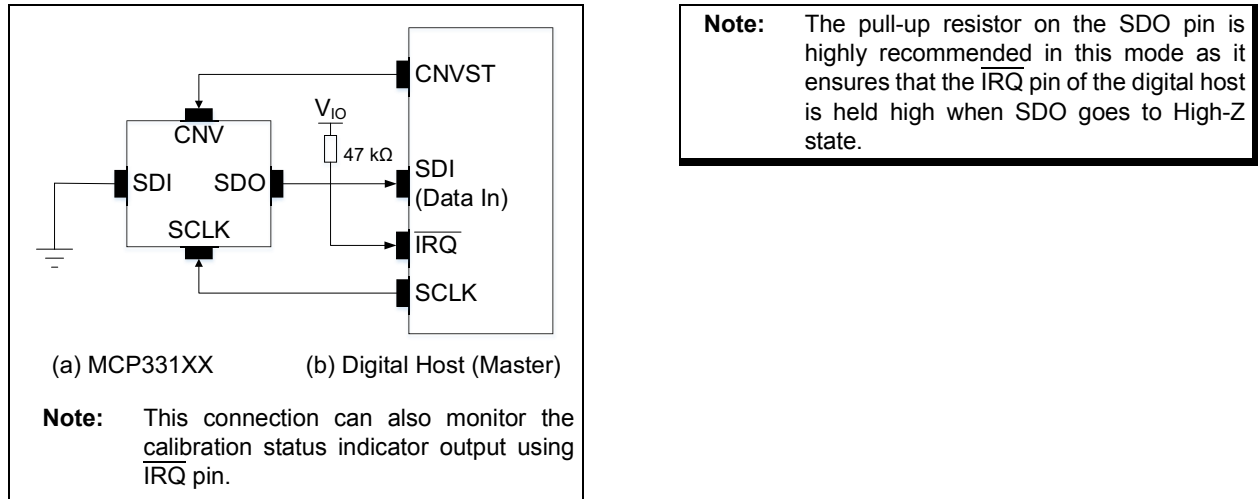
FIGURE 6-5: Connection Diagram for 3-Wire \overline{CS} Mode with BUSY Status Indicator Output Bit. \overline{IRQ} Pin in the Host Device Is Used for Interrupt Event.
