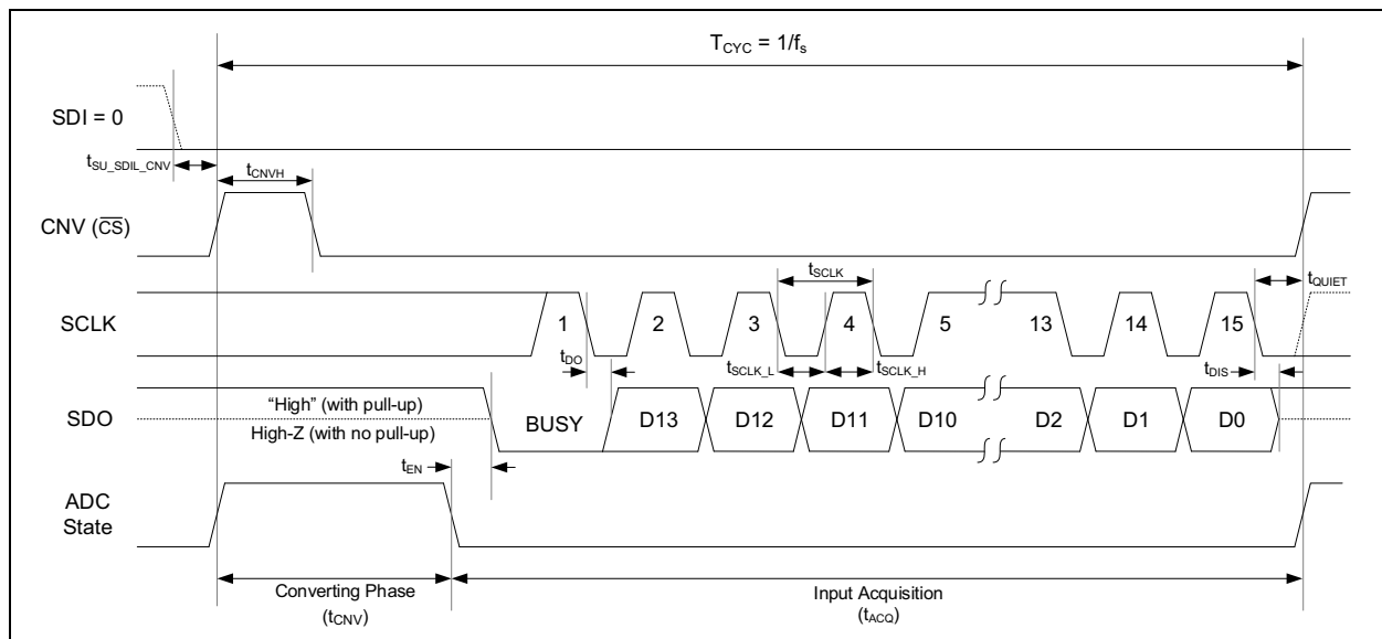
FIGURE 6-6: Timing Diagram for 3-Wire \overline{\text{CS}} Mode with \text{BUSY} Status Indicator Output Bit, Early CNV (Recommended).
