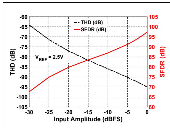
FIGURE 2-28: THD/SFDR vs. Input Amplitude: V_{REF} = 2.5\text{V} .
