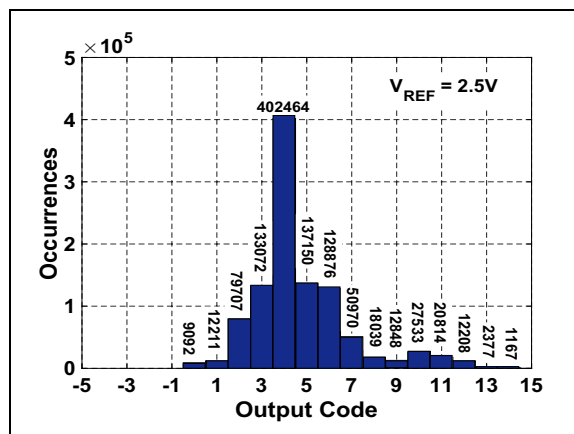
FIGURE 2-29: Shorted Input Histogram: V_{REF} = 2.5\text{V} .
