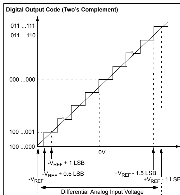
FIGURE 6-11: Ideal Transfer Function for Fully-Differential Input Signal.
