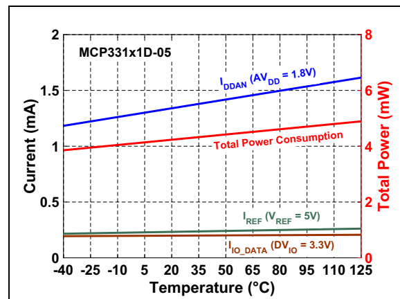
FIGURE 3-36: Power Consumption vs. Temperature: C_{LOAD\_SDO} = 20\text{ pF} .
