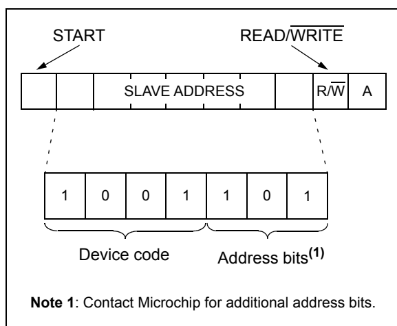
FIGURE 5-2: Device Addressing.
