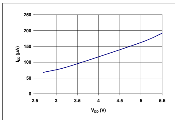
FIGURE 2-30: I_{DD} (Conversion) vs. V_{DD} .
