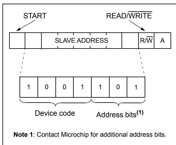
FIGURE 5-2: Device Addressing.
