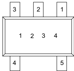
5-Pin SOT-23
