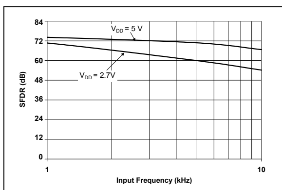
FIGURE 2-26: SFDR vs. Input Frequency.
