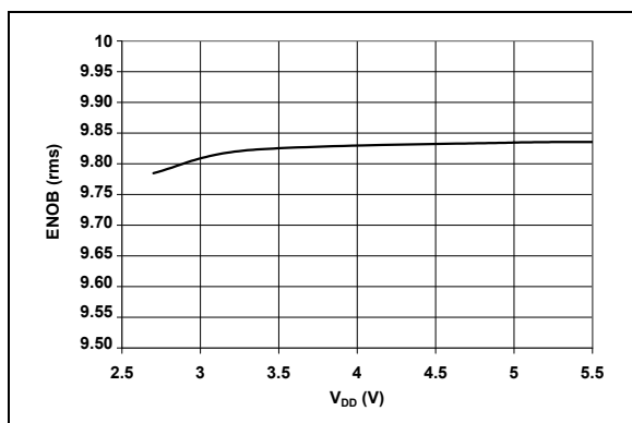
FIGURE 2-25: ENOB vs. V_{DD} .
