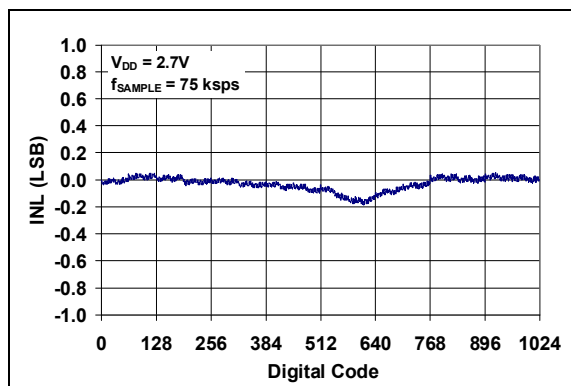
FIGURE 2-5: Integral Nonlinearity (INL) vs. Code ( V_{DD} = 2.7V ).
