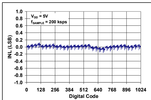
FIGURE 2-2: Integral Nonlinearity (INL) vs. Code.
