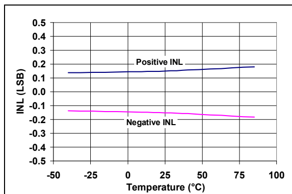
FIGURE 2-3: Integral Nonlinearity (INL) vs. Temperature.
