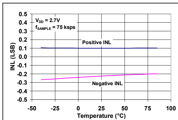
FIGURE 2-6: Integral Nonlinearity (INL) vs. Temperature ( V_{DD} = 2.7V ).
