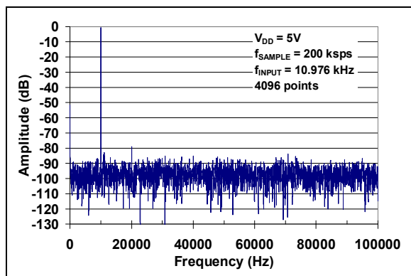
FIGURE 2-26: Frequency Spectrum of 10 kHz input (Representative Part).
