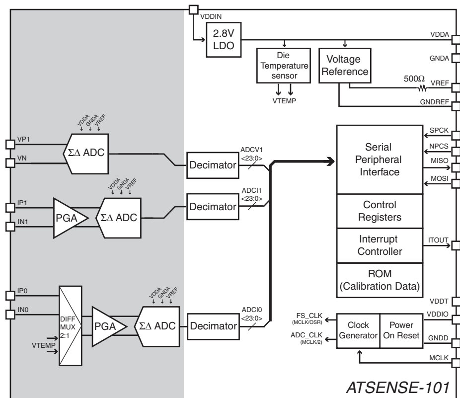
Figure 1-3: ATSENSE-101 Functional Block Diagram
